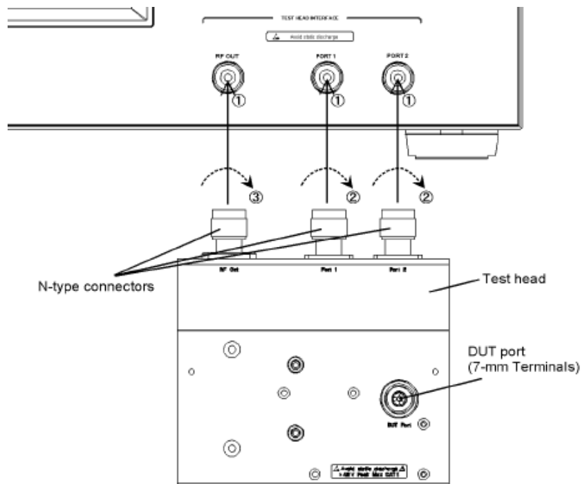
Figure 3 Connecting Test head to E4991B
