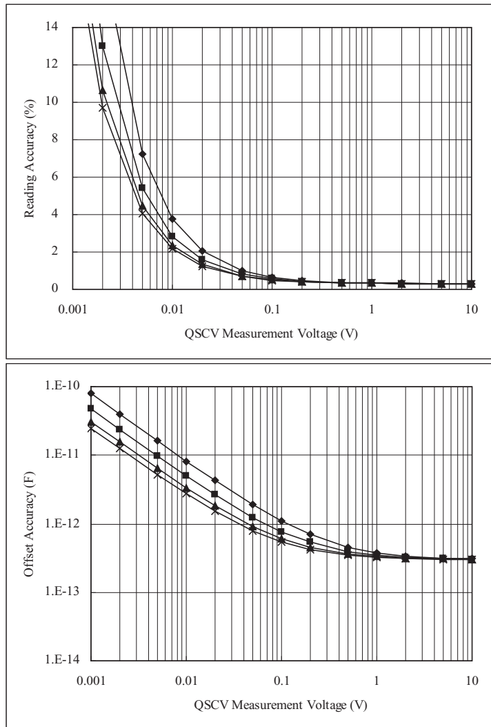
Calculation Example of Measurement Accuracy: HRSMU, ASU+SMU
