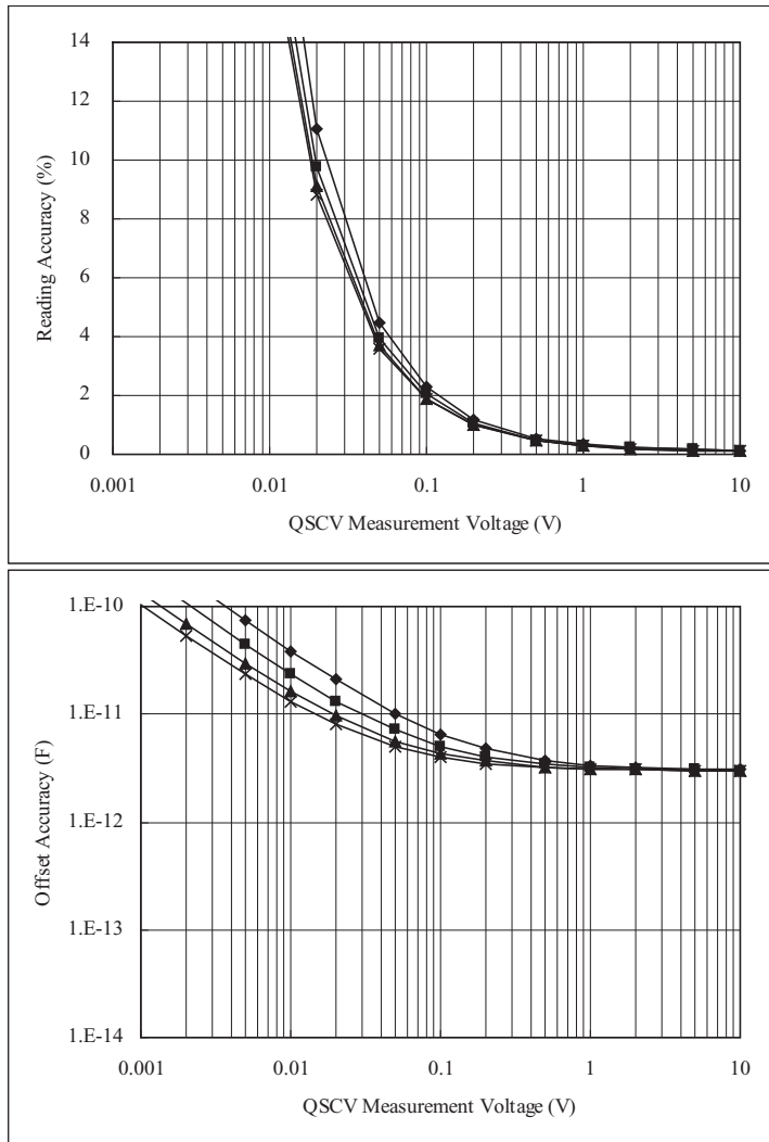
Calculation Example of Measurement Accuracy: MP/HRSMU, ASU+SMU
