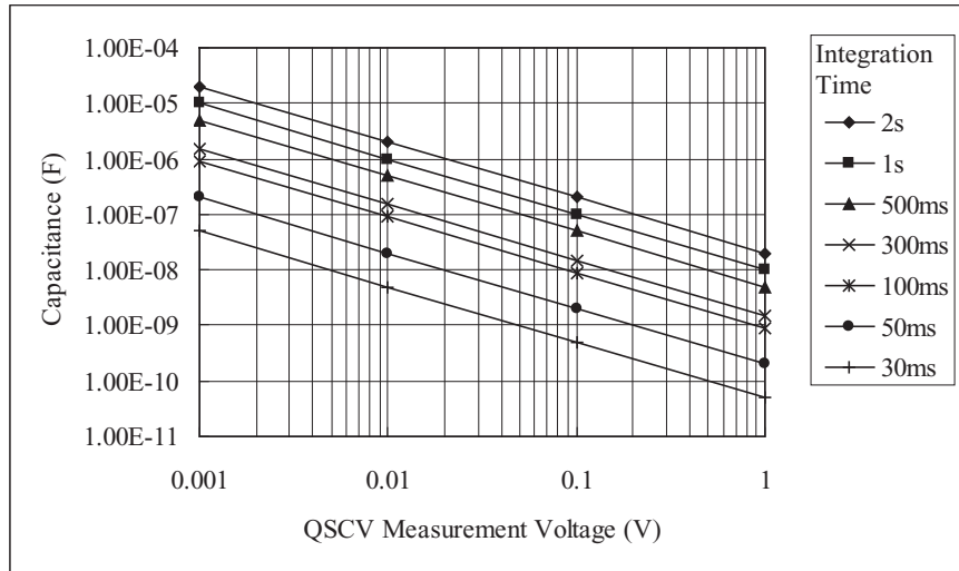
Maximum Measurement Value Using 10 nA Range: HPSMU, MPSMU, HRSMU, ASU+SMU
