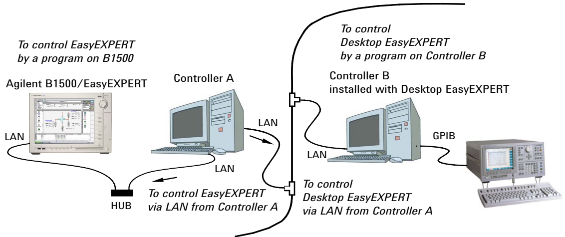
Figure 6-1 Image of EasyEXPERT Remote Control
