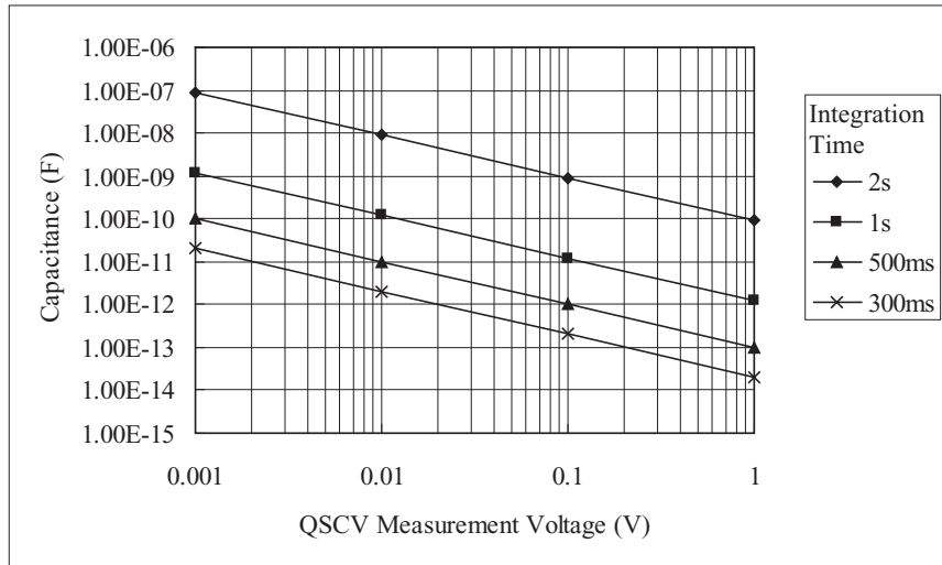
Figure 8-1 Maximum Measurement Value Using 10 pA and 100 pA Range: HRSMU, ASU+SMU
