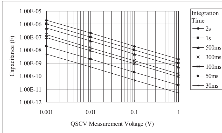
Figure 8-2 Maximum Measurement Value Using 1 nA Range: HPSMU, MPSMU, HRSMU, ASU+SMU
