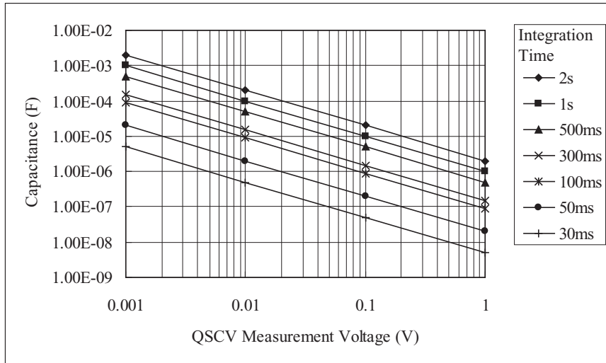
Maximum Measurement Value Using 1 \mu A Range: HPSMU, MPSMU, HRSMU, ASU+SMU
