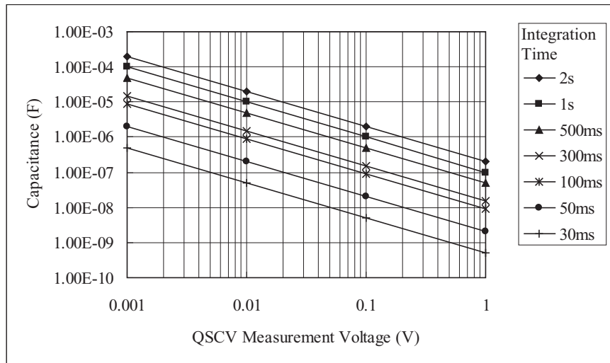
Maximum Measurement Value Using 100 nA Range: HPSMU, MPSMU, HRSMU, ASU+SMU
