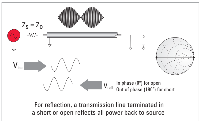
Figure 9. Transmission line terminated with short, open
