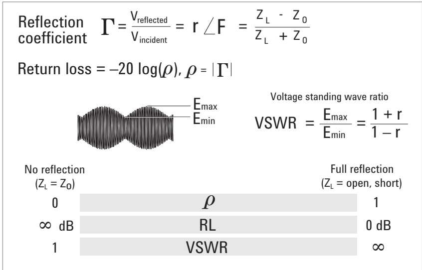
Figure 11. Reflection parameters
