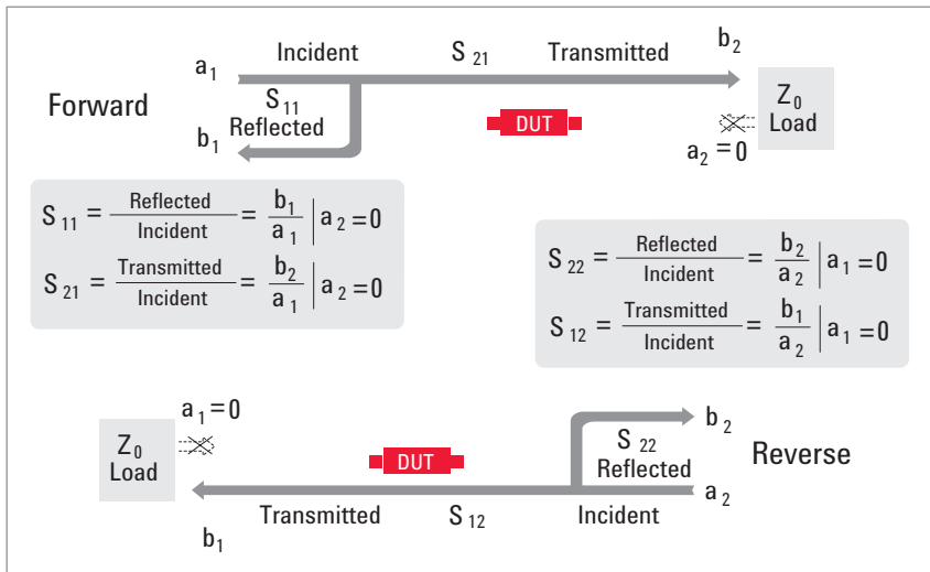
Figure 17. Measuring S-parameters
