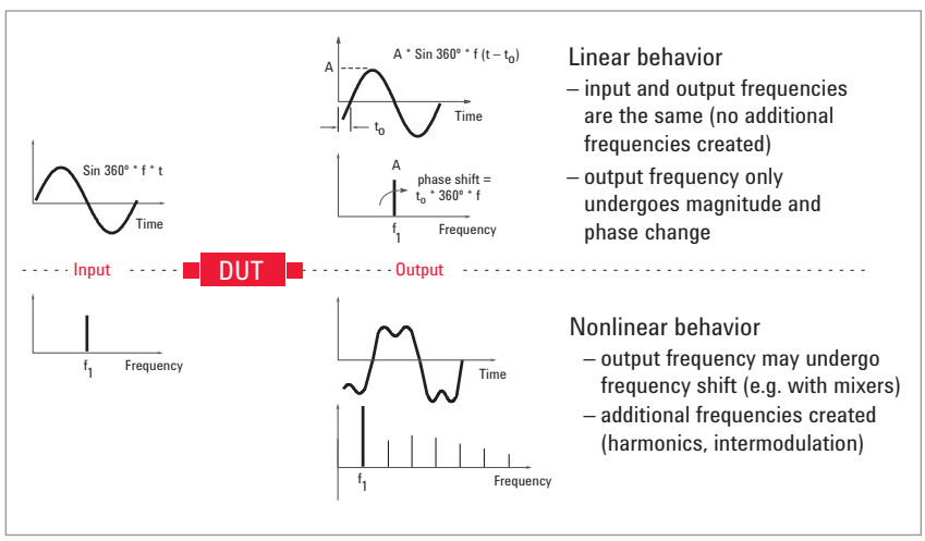
Figure 1. Linear versus nonlinear behavior
