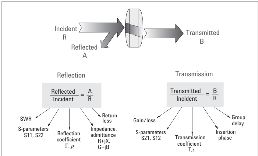
Figure 10. Common terms for high-frequency device characterization
