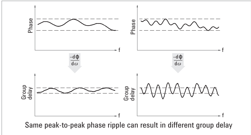
Figure 15. Why measure group delay?
