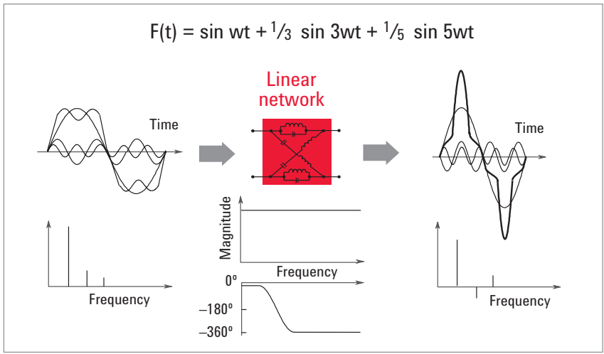
Figure 3. Phase variation with frequency
