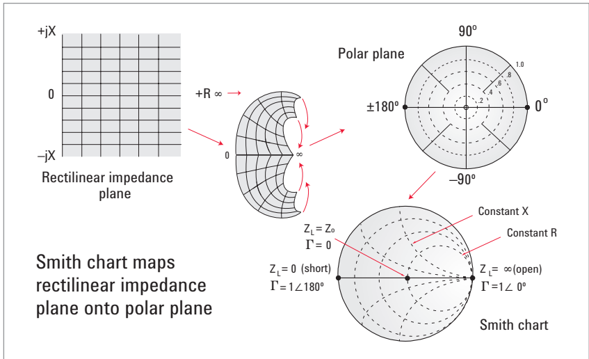
Figure 6. Smith chart review
