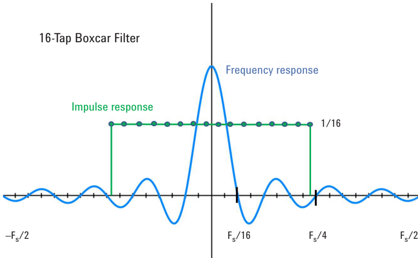
Figure 5. Impulse and frequency response for a 16-tap boxcar-averaging filter
