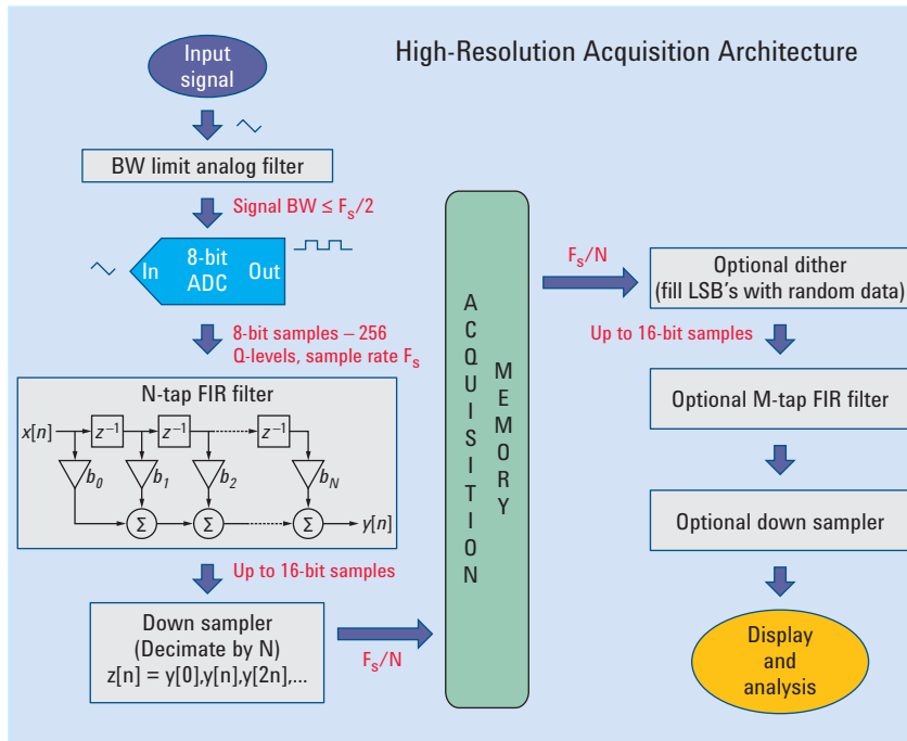
Figure 4. High-resolution acquisition architecture
