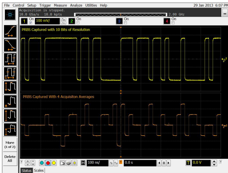
Figure 6. High resolution works great for capturing a low-noise PRBS signal, while averaging does not
