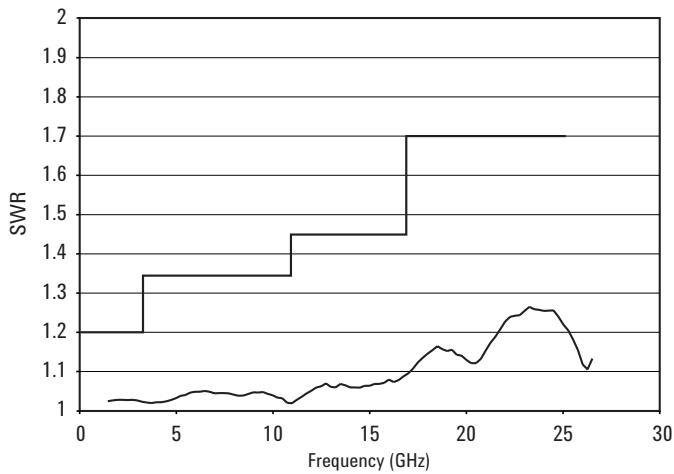
Figure 13. Keysight L-Series multiport switch SWR versus frequency
