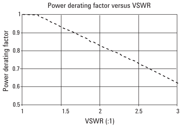
Figure 9. Power derating factor versus VSWR
