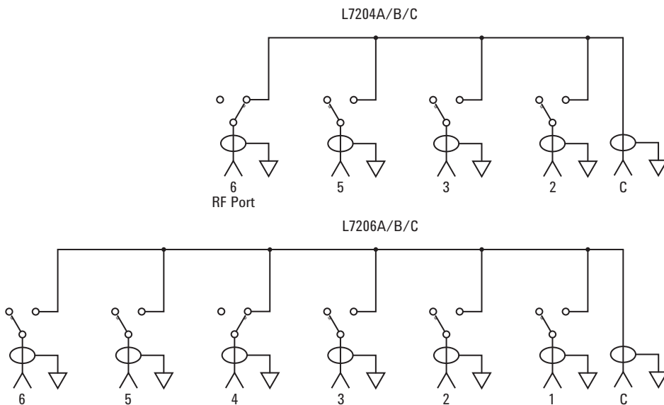
Figure 2. Keysight L7204A/B/C and L7206A/B/C unterminated simplified schematics
