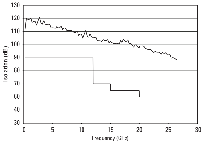
Figure 12. Keysight L-Series multiport switch isolation versus frequency
