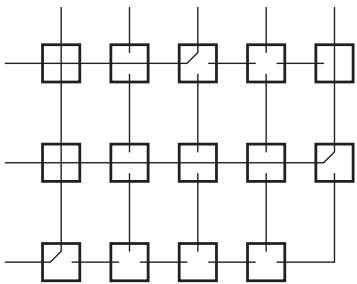
Figure 5. Cross-point matrix
