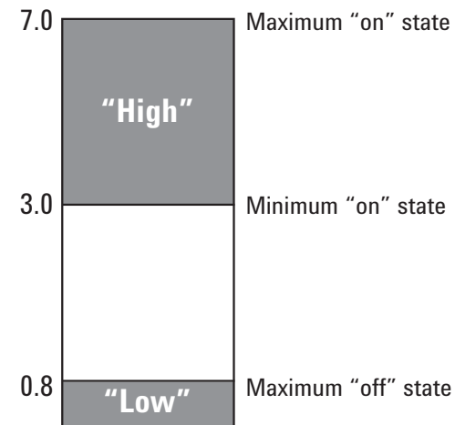
Figure 10. TTL control voltage states (Option T24)
