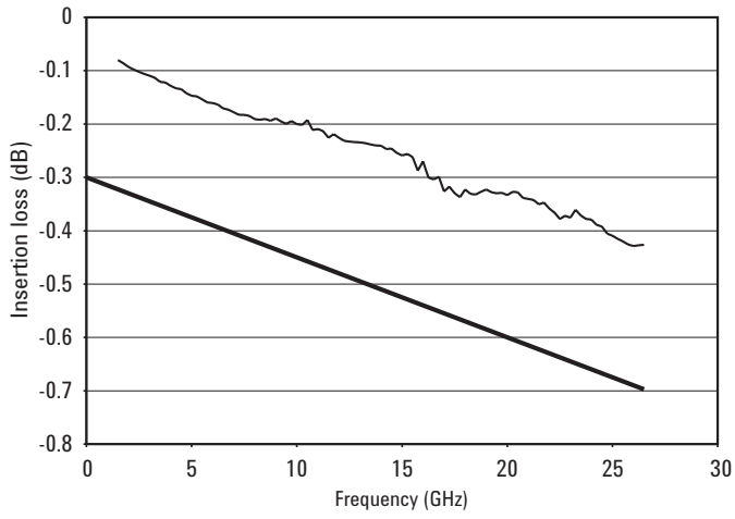
Figure 11. Keysight L-Series multiport switch insertion loss versus frequency
