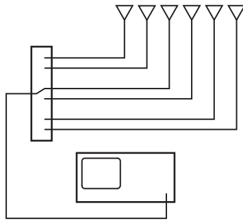
Figure 4. Multiport matrix
