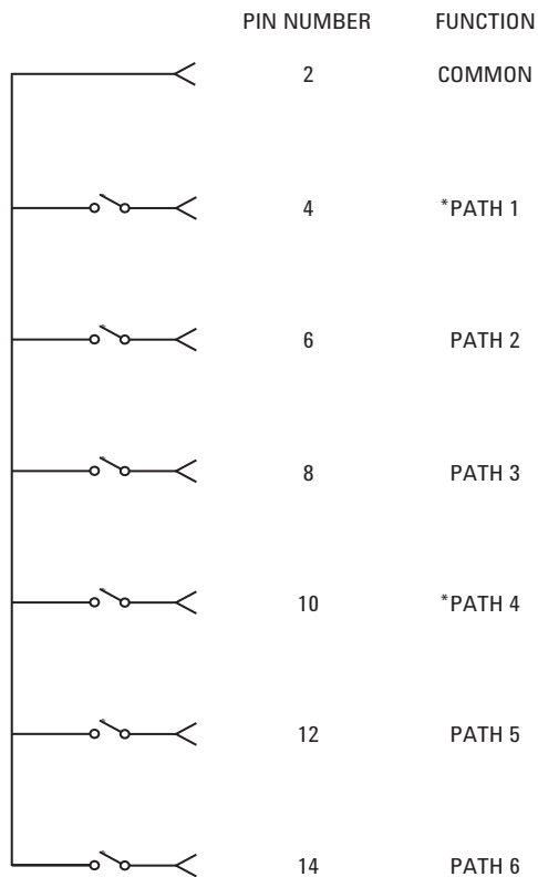
Figure 7. Pin function diagram
