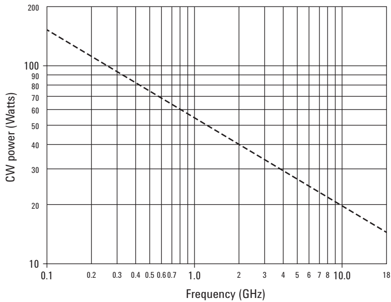
Figure 8. Power rating for cold switching at 75 °C
