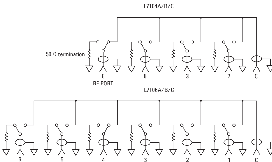
Figure 1. Keysight L7104A/B/C and L7106A/B/C simplified schematics
