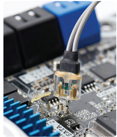
Figure 7. Use InfiniiMax III+ probe amplifier with QuickTip head for quick and secure magnetic connection.
