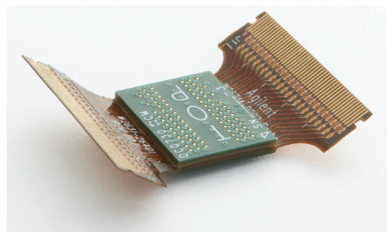
Figure 9. DDR2 BGA probe adapter for oscilloscopes and logic analyzers
