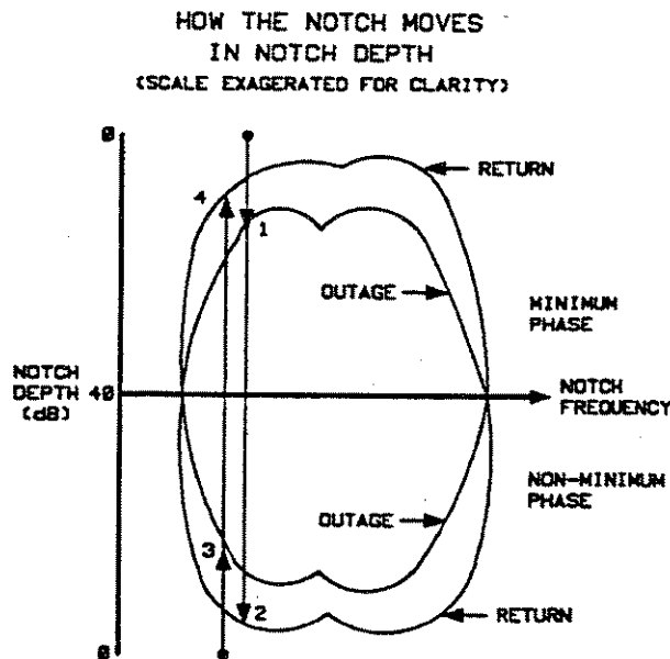
Figure 2-5. Hysteresis-M Measurement
