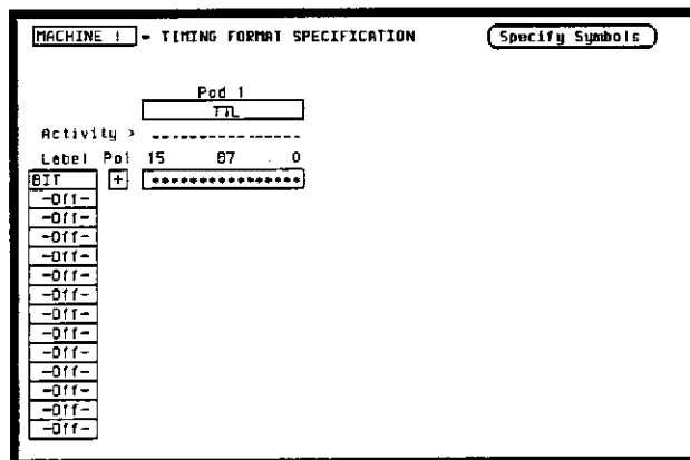
Figure 3-3 Pod Threshold
