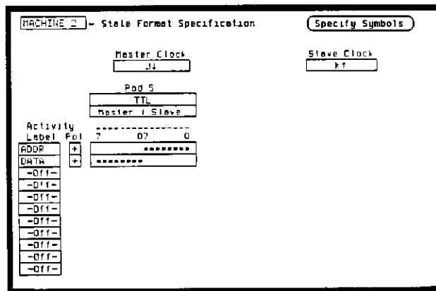
Figure 5-49. Bit Assignments for Master and Slave Clocks
