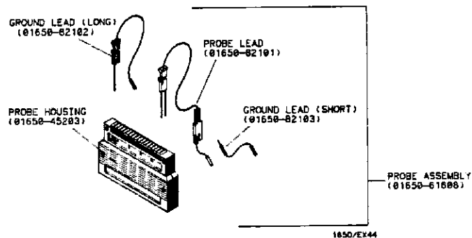
Figure 12-3 Probe Assembly
