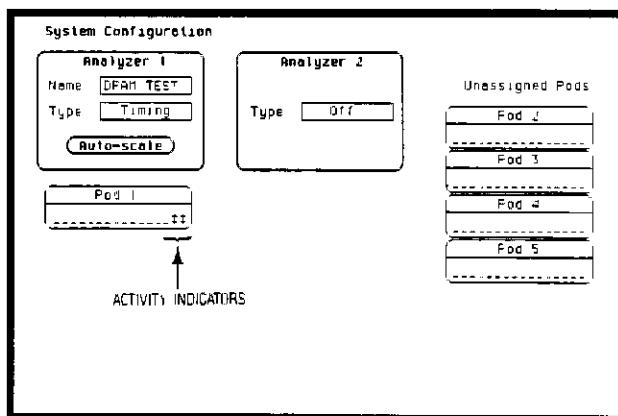
Figure 7-3. Activity Indicators
