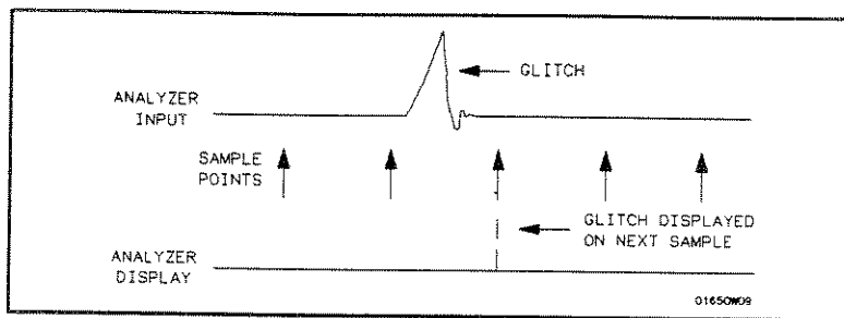
Figure 10-5. Glitch in Timing Waveform
