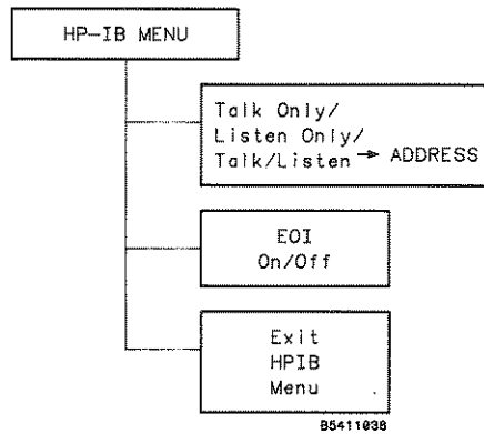
Figure 6-18. HP-IB Menu
