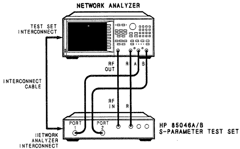
Figure 4-4. Switch Repeatability Test Setup
