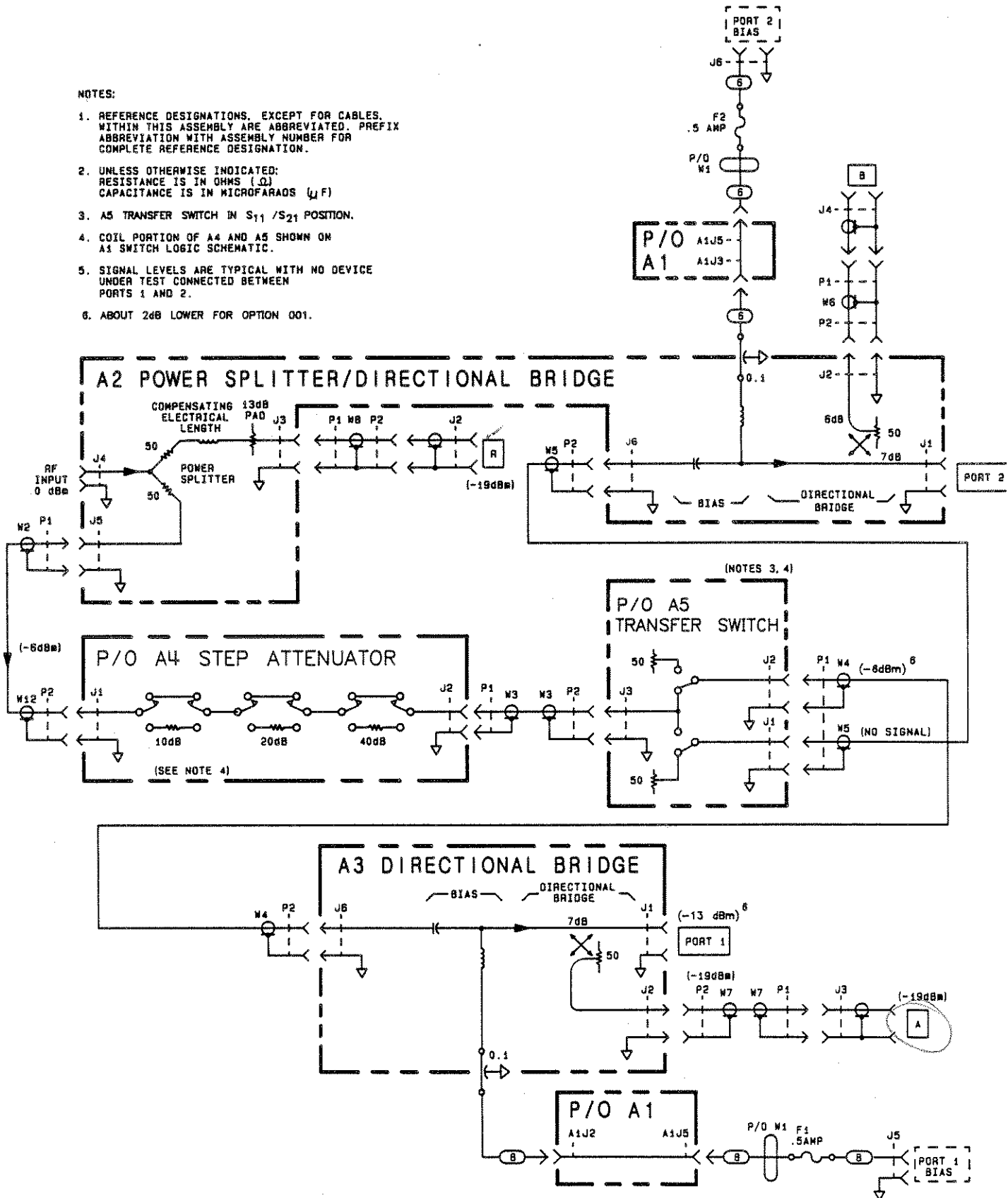
Figure 8-3. Schematic Diagram
