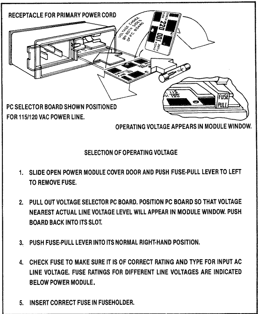
FIGURE 3. VOLTAGE SELECTION WITH POWER MODULE PC BOARD
