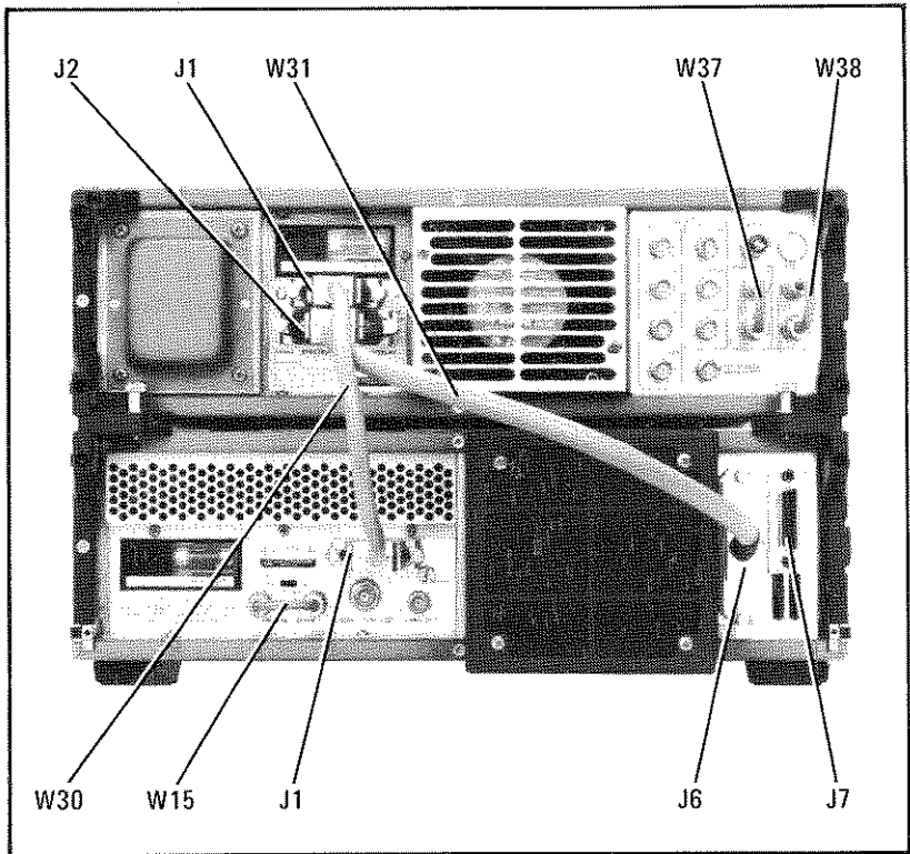
FIGURE 2. REAR PANEL WITH INTERCONNECT CABLES INSTALLED
