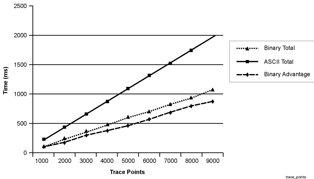
Figure 2 Binary vs. ASCII Downloads
