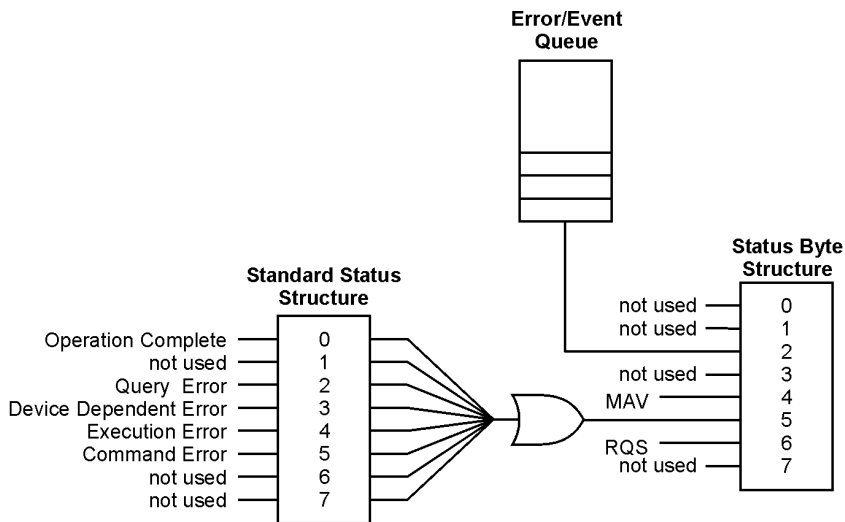
Figure 1 Status Registers
