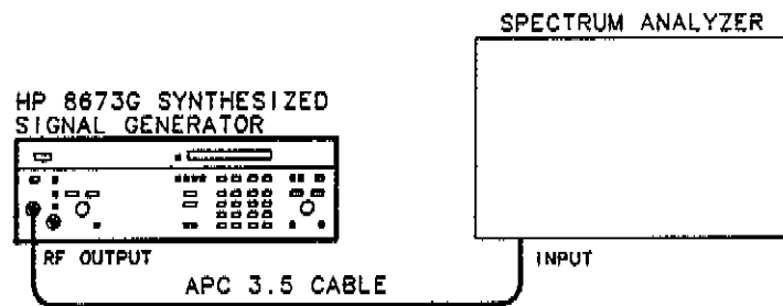
Figure 4-12. Harmonics, Subharmonics, and Multiples Test Setup
