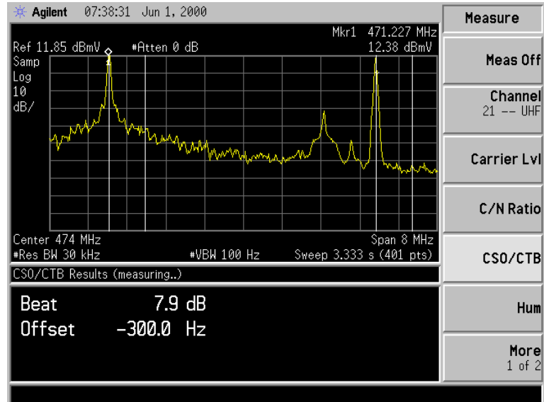
Figure 2-10 CSO/CTB Measurement (PAL-B/G)
