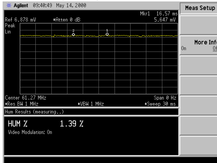
Figure 2-11 Hum Measurement (NTSC-M)
