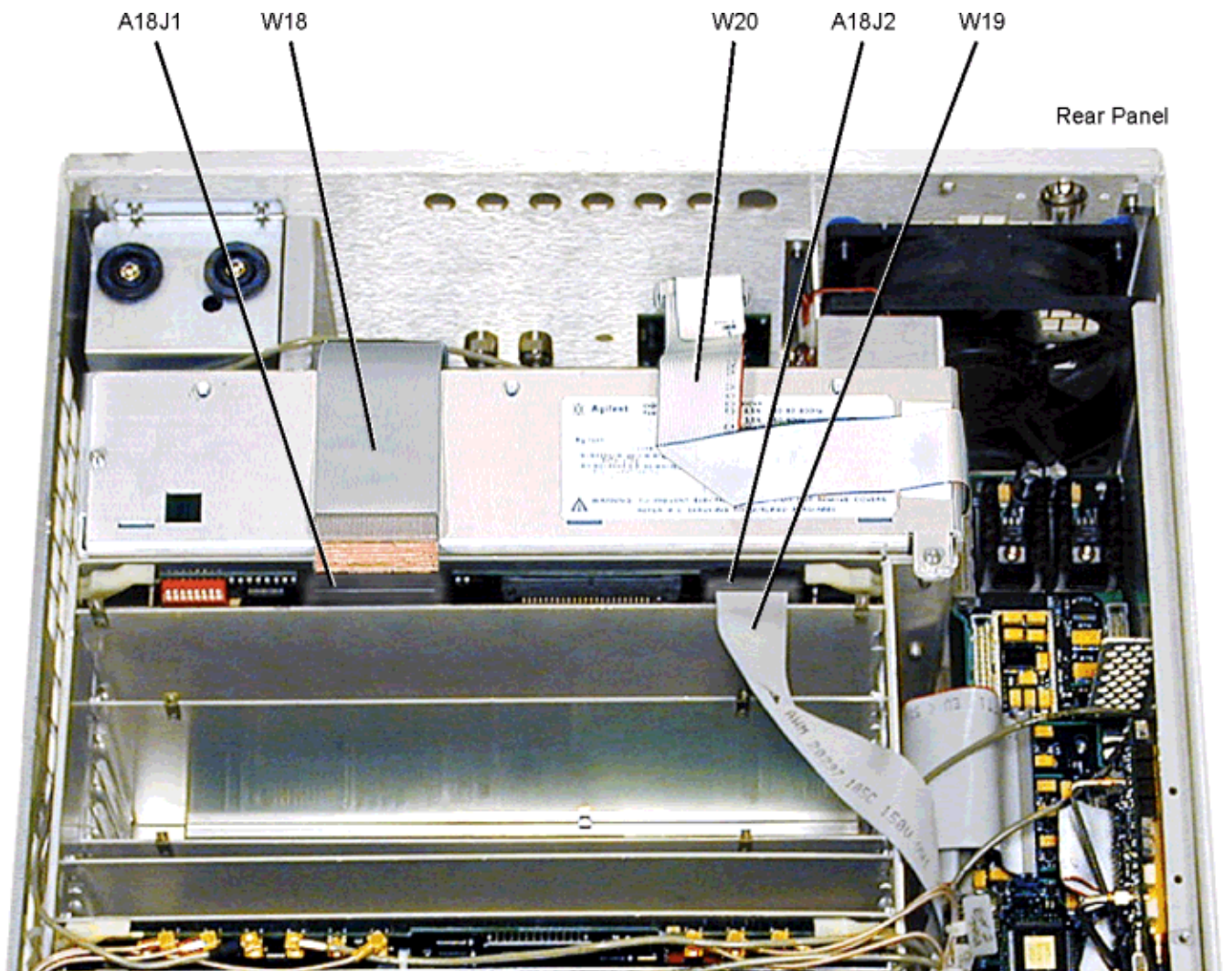
Figure 2-16 A18 CPU
