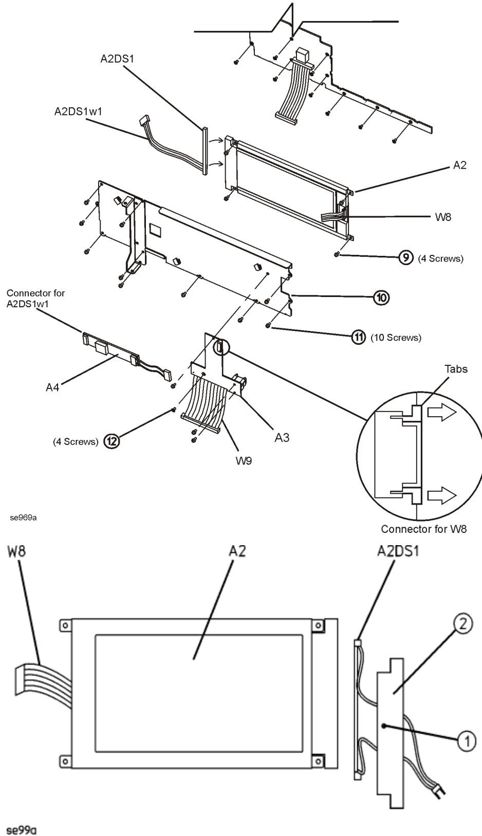
Figure 2-6 A2DS1 Display Backlight Removal
