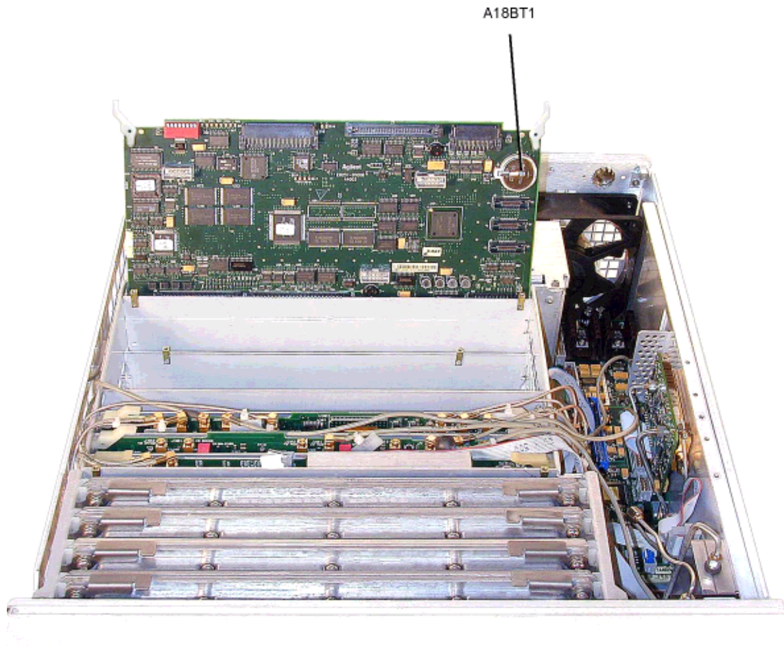
Figure 3-7 Battery-Lithium
