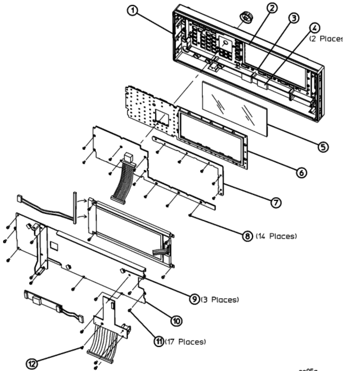
Figure 3-16 Disassembled Front Panel View
