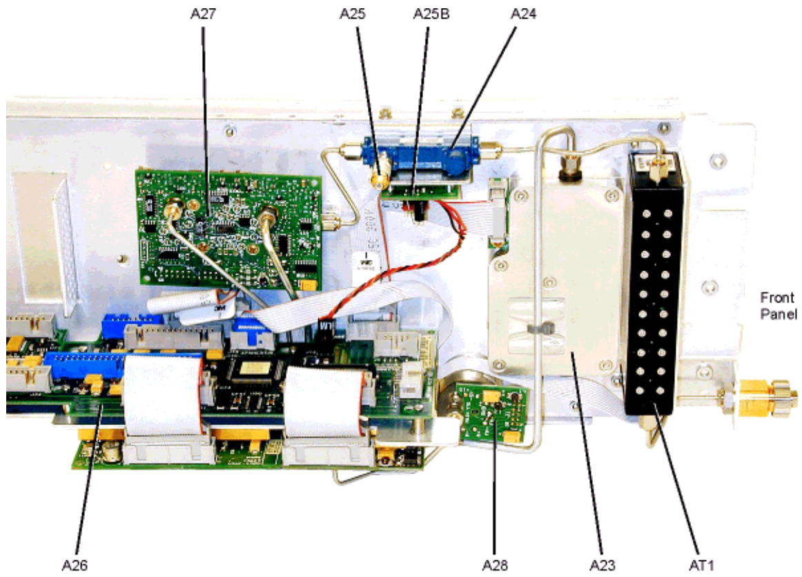
Figure 2-28 A25 40 GHz High Band Detector with Bias Board
