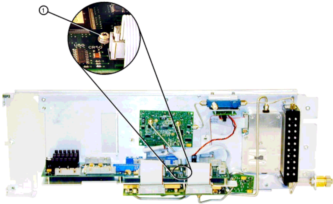
Figure 3-22 Microcircuit Interface Deck Top View
