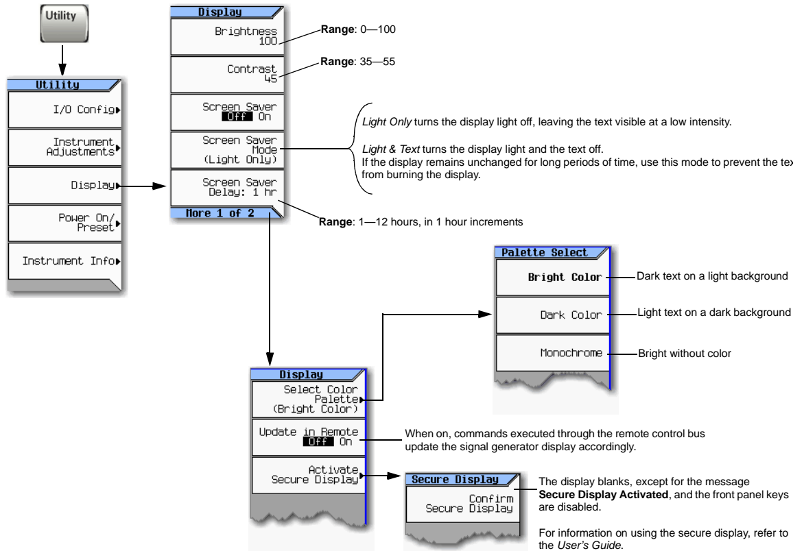
Figure 2-2 Display Softkeys
