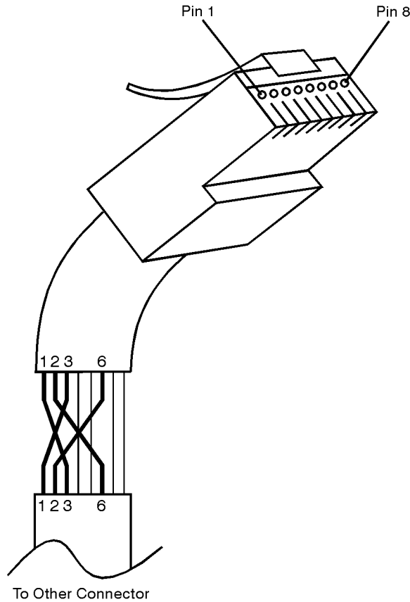
Figure 5-2 Cross-Over Patch Cable Wiring (cross-over end)
