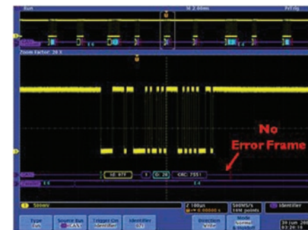
Turning on serial decoding severely limits the update rate of the Tektronix MDO4000 Series as it is not able to capture the error frame
