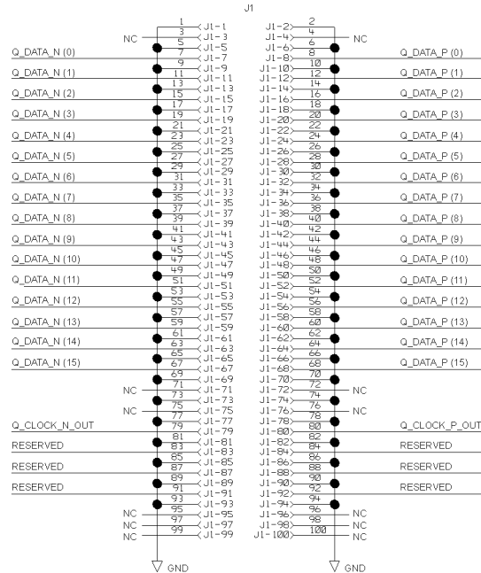
Figure 3-5 Dual 100-Pin Samtec Connector
