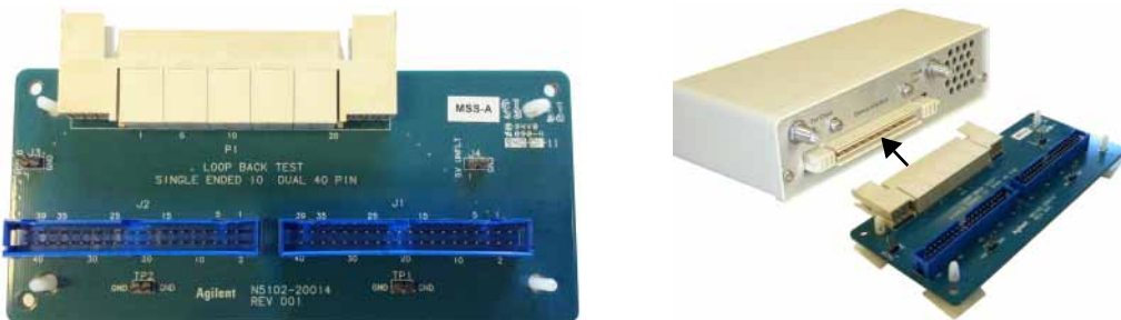
Figure 1-5 Connecting the Loop Back Board to the N5102A Module
