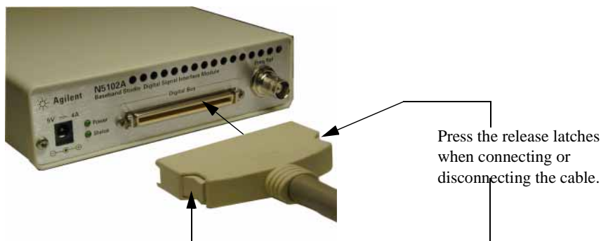
Figure 1-2 N5102A Module Digital Bus Cable Connection
