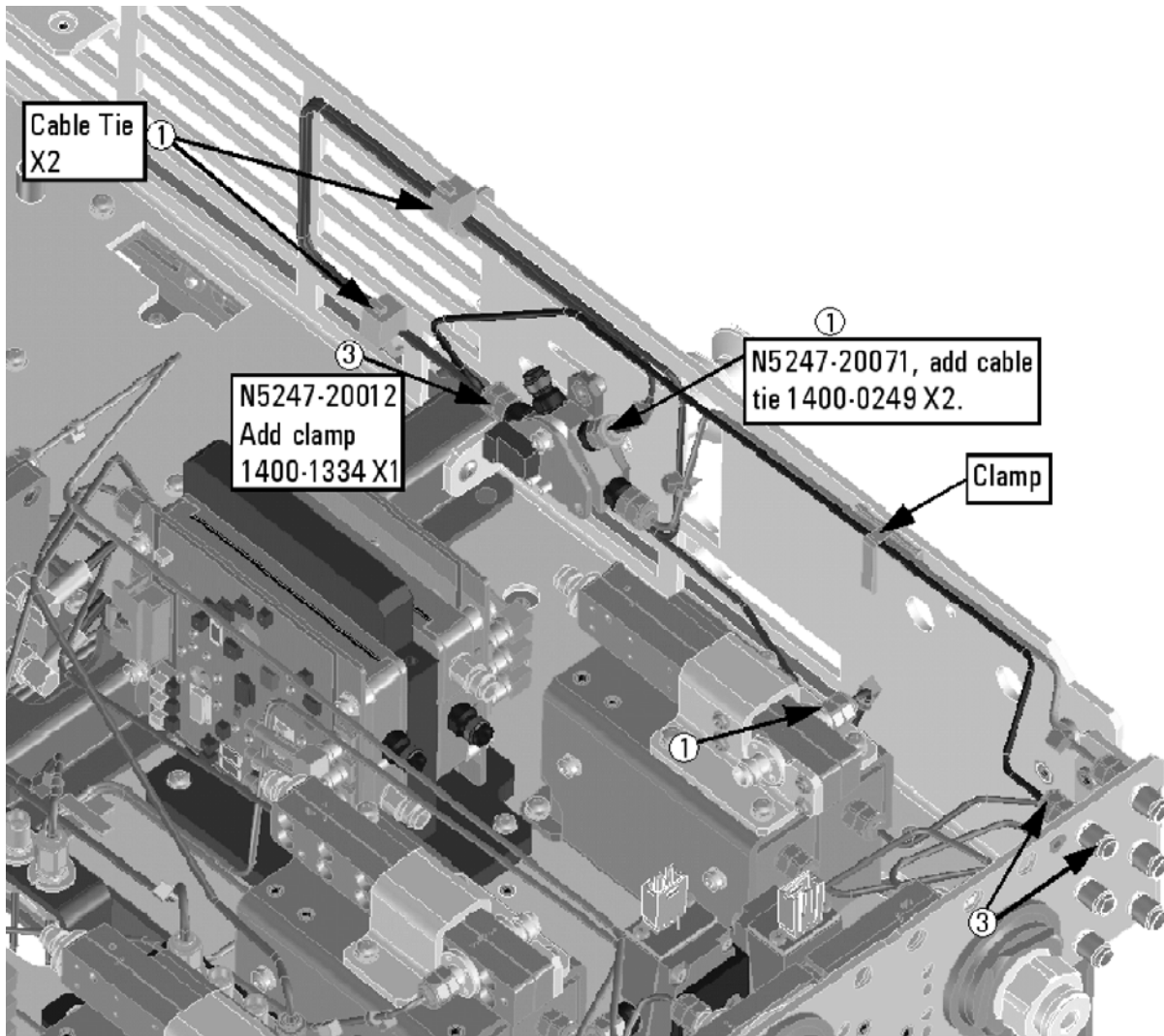
Figure 31 Location of Cable Tie to Secure W144
