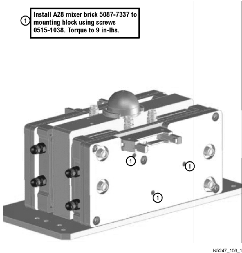
Figure 15 A28 Mixer Brick Assembly
