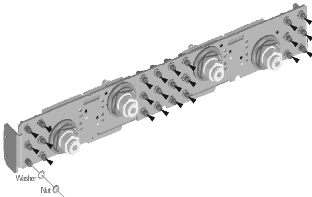
Figure 25 Bulkhead Connectors Installation
