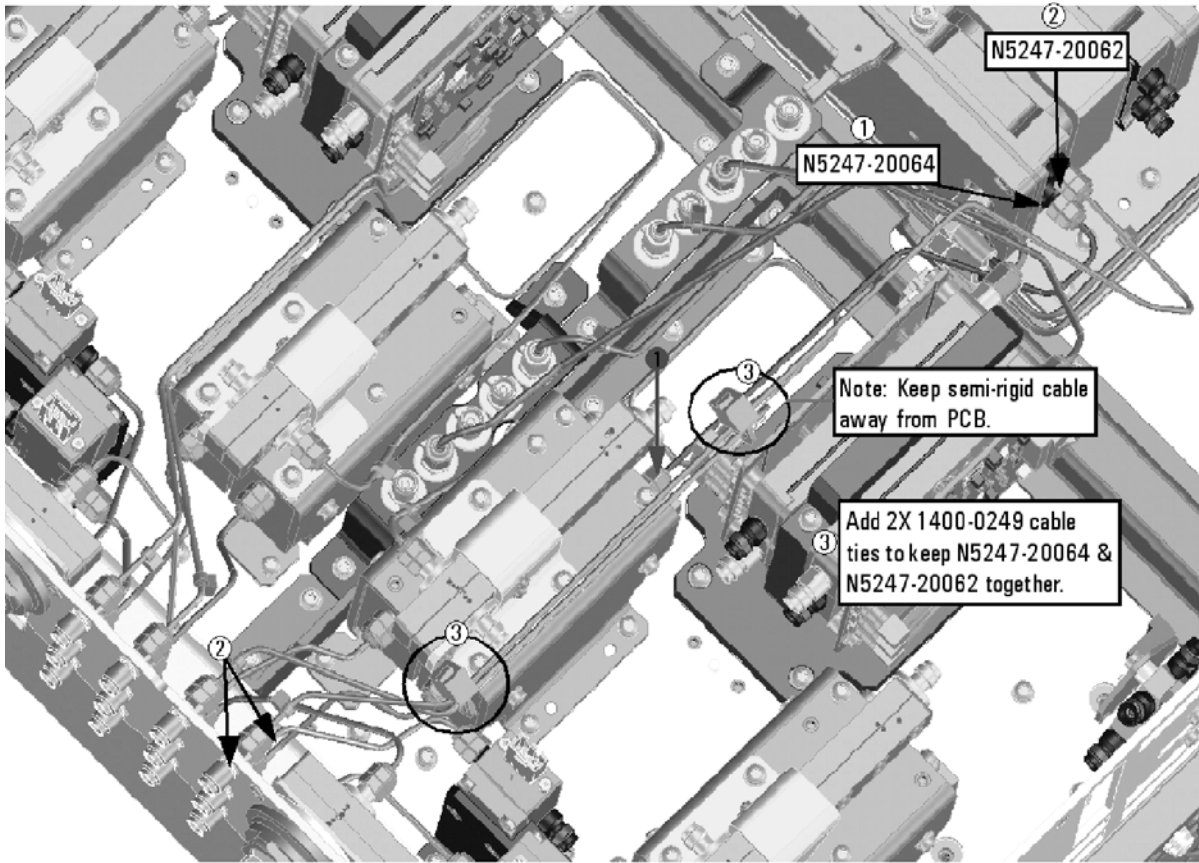
Figure 30 Location of Cable Ties to Secure W120/W54
