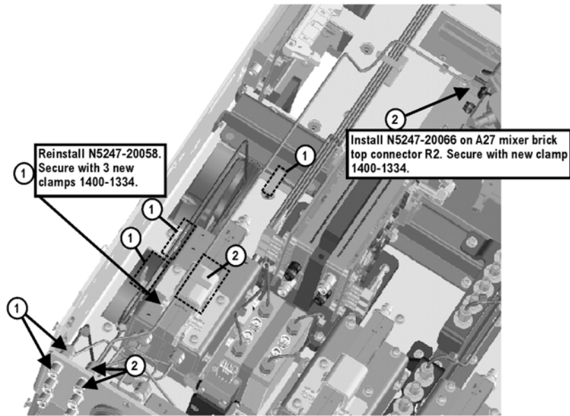
Figure 27 Location of W45 and W145 Cable Securing Clamps
