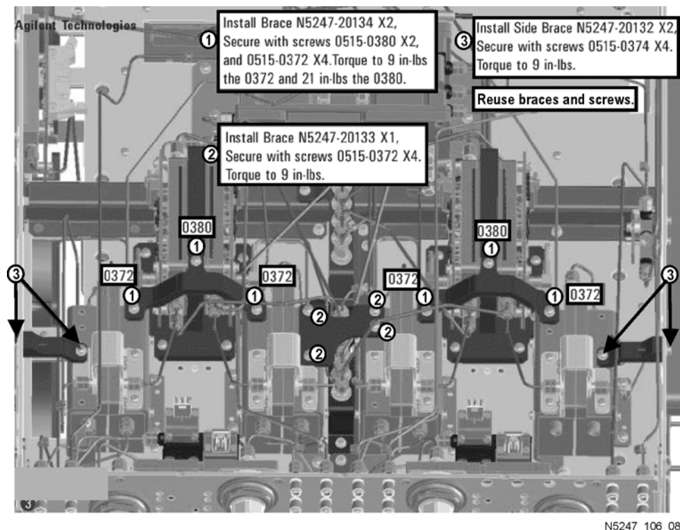
Figure 32 Location of Braces on the Bottom Side of the PNA
