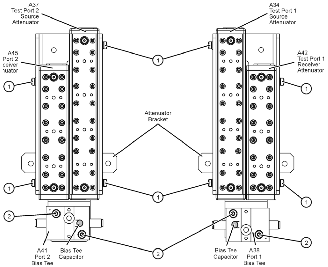
Figure 6 Step Attenuators and Bias Tees Assembly
