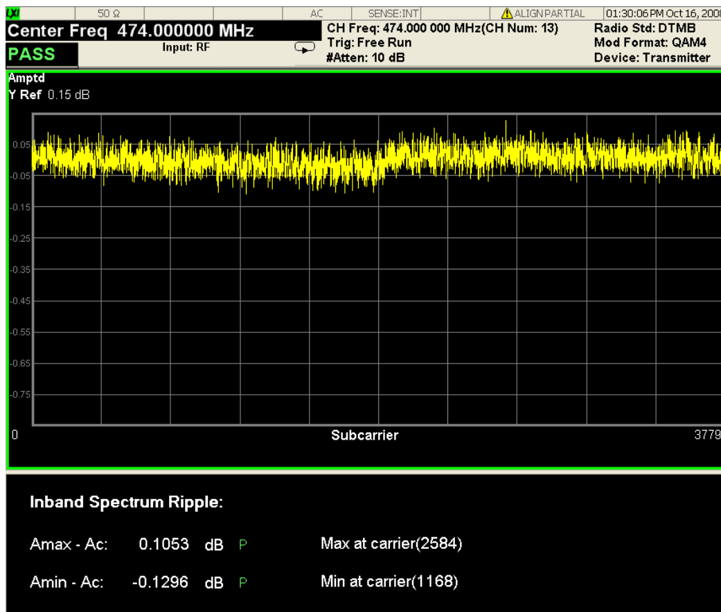
Figure 5 - 5 Spectral Flatness View of Modulation Accuracy Measurement
