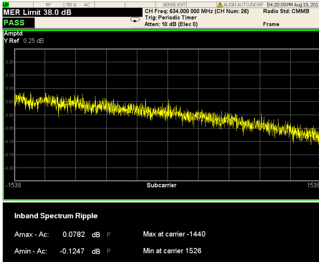
Figure 5 - 5 Spectral Flatness View of Modulation Accuracy Measurement
