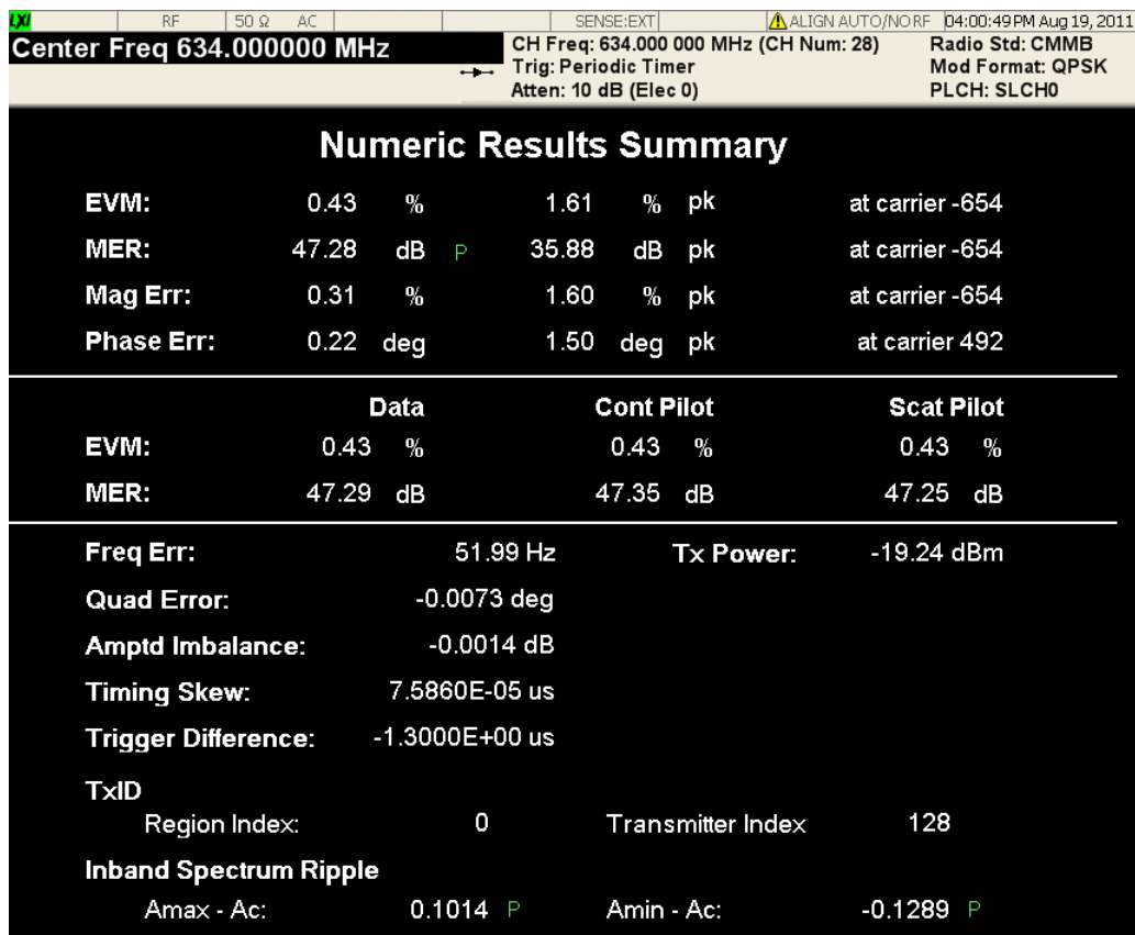
Figure 5 - 6 Result Metrics View of Modulation Accuracy Measurement
