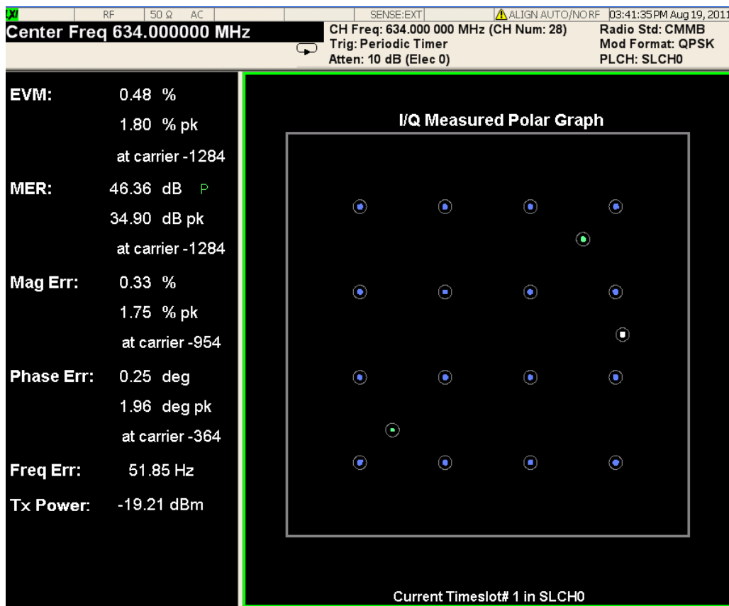
Figure 5 - 1 I/Q Measured Polar Graph View of Modulation Accuracy Measurement
