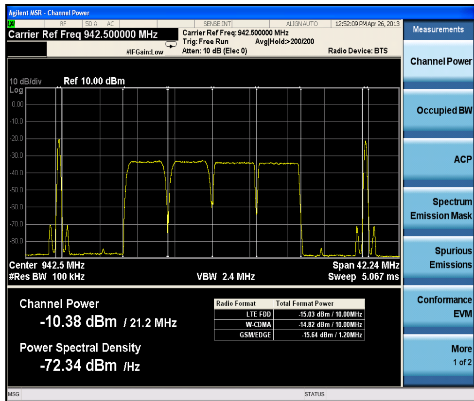
MSR Downlink Channel Power Measurement Result - Power Results View
