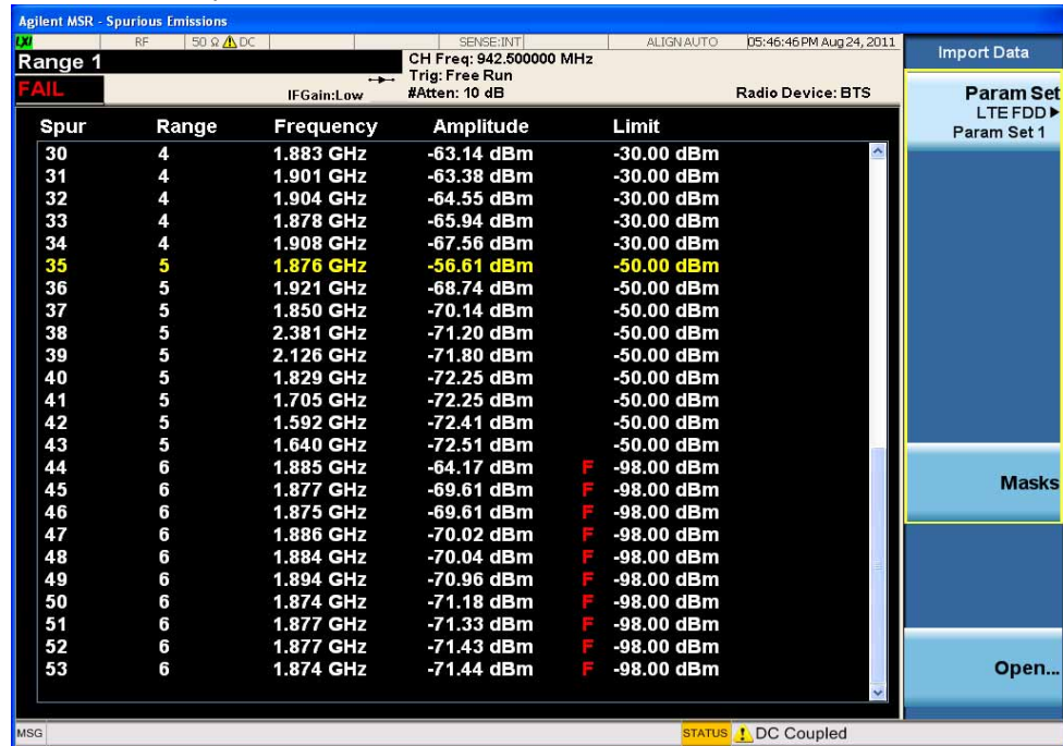
MSR Downlink Spurious Emissions Measurement - Numeric Result Screen
