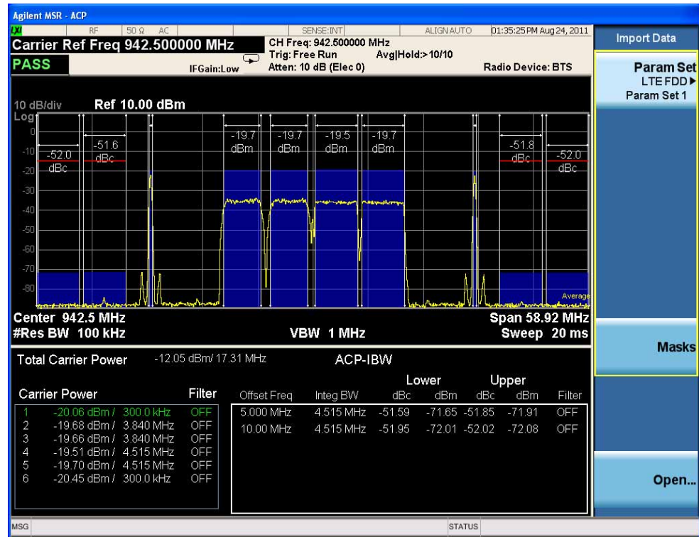
Figure 2-13 MSR Downlink ACP Measurement Result - Result Trace View
