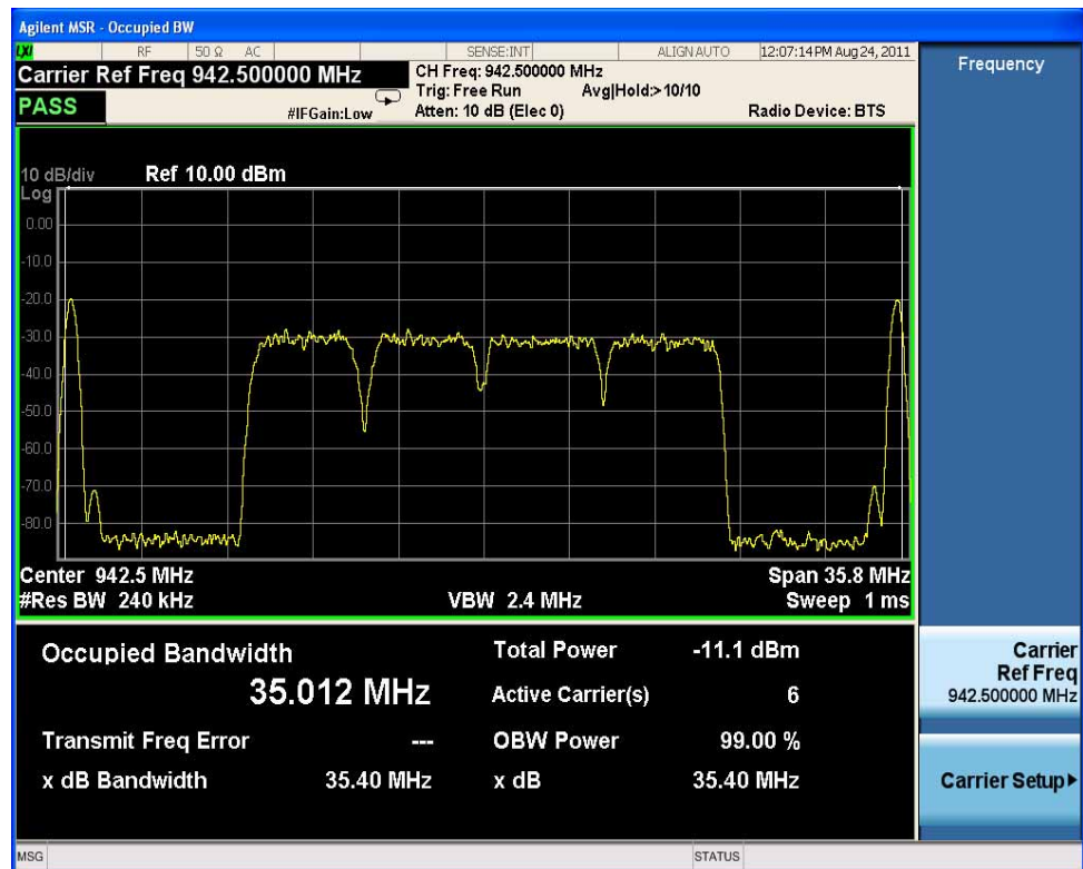
MSR Downlink Occupied BW Measurement Result
