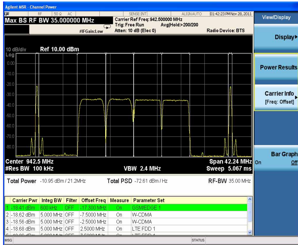
Figure 2-10 MSR Downlink Channel Power Measurement Result - Carrier Info View
