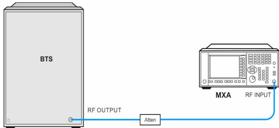
Figure 2-2 Base Station Test System
