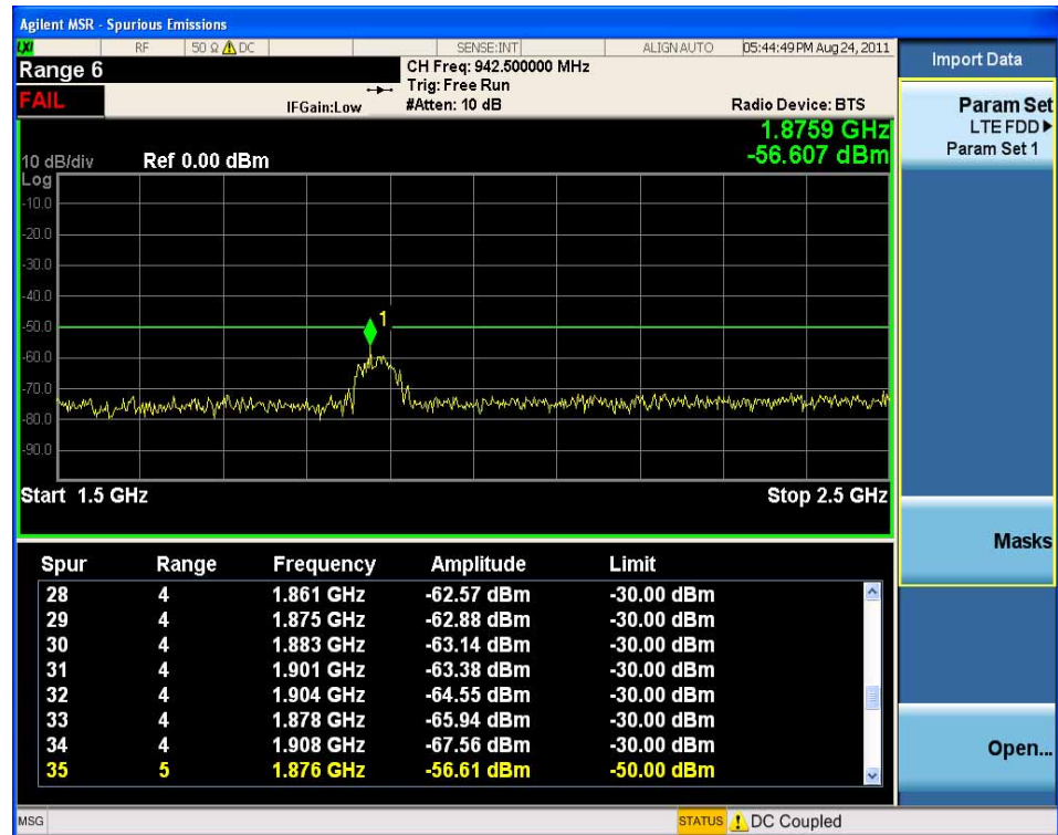
MSR Downlink Spurious Emissions Measurement - Spur Table
