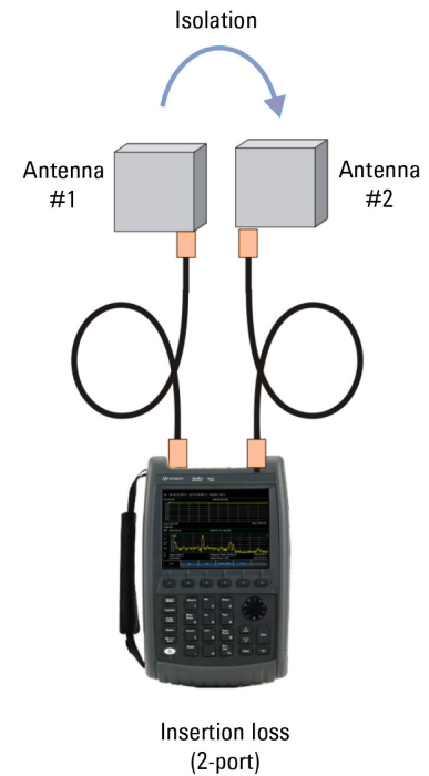
Figure 6b. Configuration for measuring antenna-to-antenna isolation
