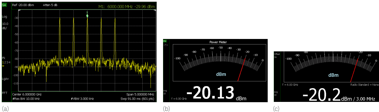
Figure 8. Measurement of a multi-tone signal using the (a) spectrum analyzer, (b) power sensor and (c) spectrum analyzer with built-in channel power meter (CPM)
