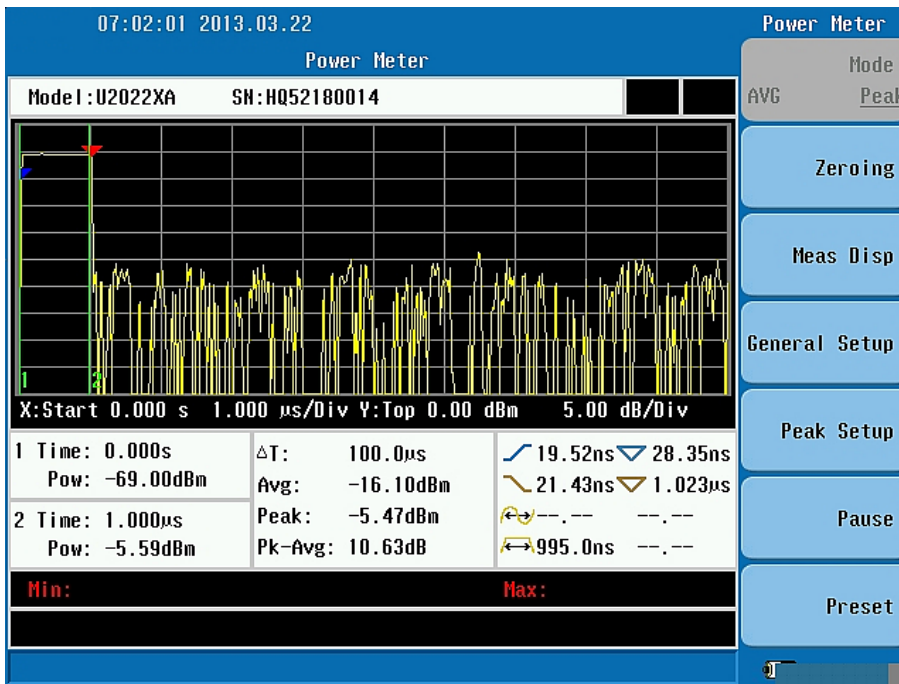
Figure 13. Measurement of a pulsed waveform using a peak power sensor connected to a spectrum analyzer
