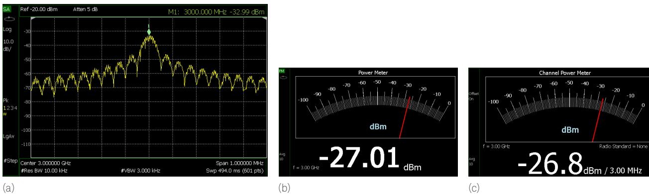
Figure 11. Measurement of a pulsed waveform with 20% duty factor using the (a) spectrum analyzer, (b) power sensor and (c) spectrum analyzer with built-in channel power meter (CPM)
