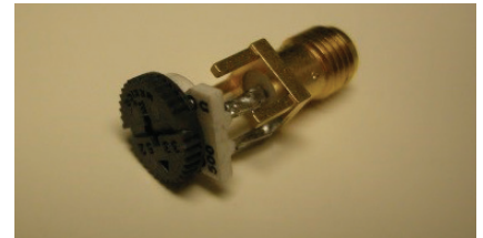
Figure 6. The variable 500 \Omega potentiometer load
