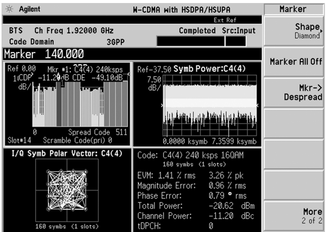
Figure 10. Code domain quad view
