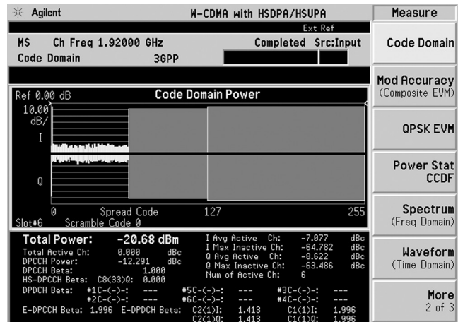
Figure 12. HSUPA uplink code domain analysis
