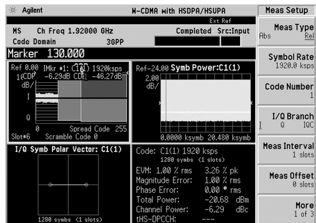
Figure 13. Symbol analysis of E-DPDCH in spreading factor 2 (1920 ksps)
