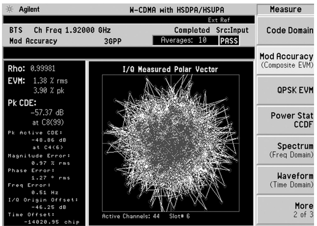
Figure 15. Modulation accuracy of HSDPA signal
