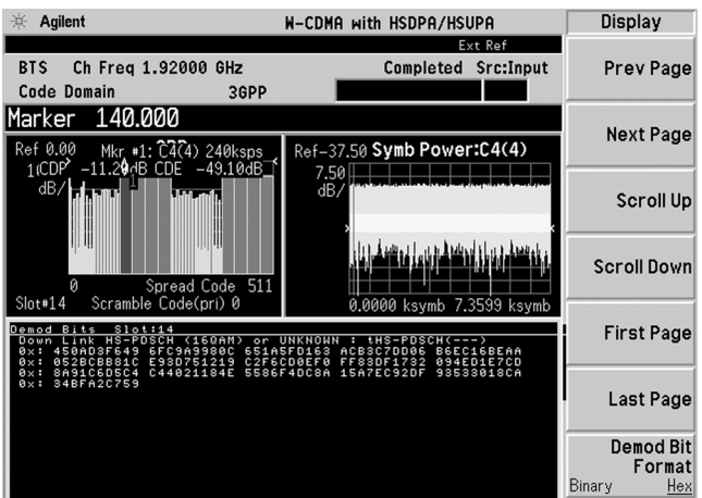
Figure 11. Demodulated bits in hexadecimal
