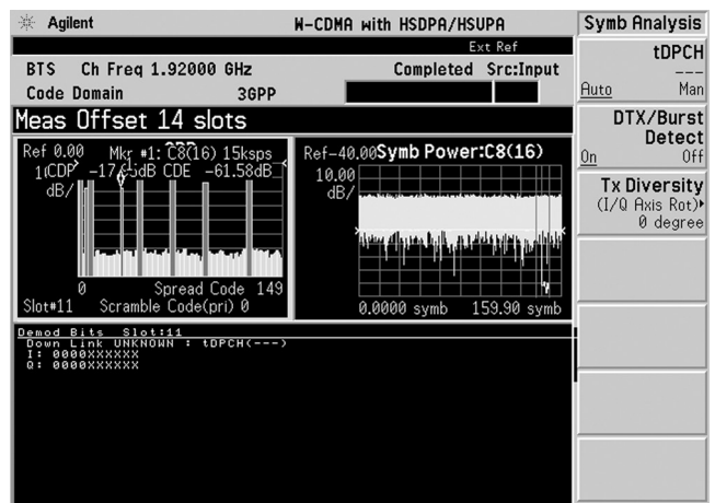
Figure 8. Symbol power and demodulated I/Q bits
