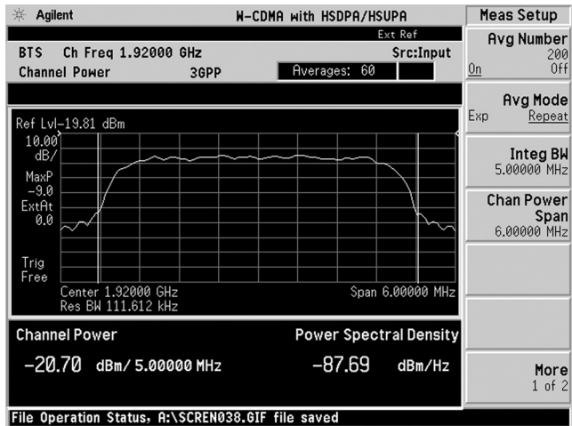
Figure 1. Channel power
