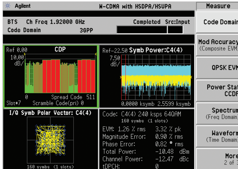
Code domain analysis for a W-CDMA with HSDPA PSA Series spectrum analyzer with Options BAF and 210
