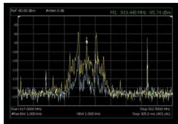
Figure 3: This over-the-air measurement, performed using FieldFox, compares the received signal using an omnidirectional antenna (blue trace) and a high-gain antenna (yellow trace). There is a noticeable increase in the measured amplitude of the unknown signal when using the high-gain antenna, but this measurement required the antenna to be pointed in the direction of the highest signal amplitude.
