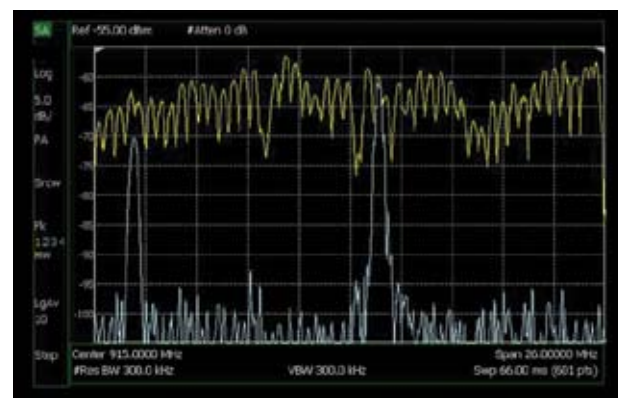
Figure 2: The measurement of a frequency hopping signal is displayed here in FieldFox's standard Clear/Write (blue trace) and MaxHold (yellow trace) modes. During measurement, the signal to the left was observed to be stationary and could represent a source of interference to the hopping signal when the two signals eventually collide in the frequency domain.
