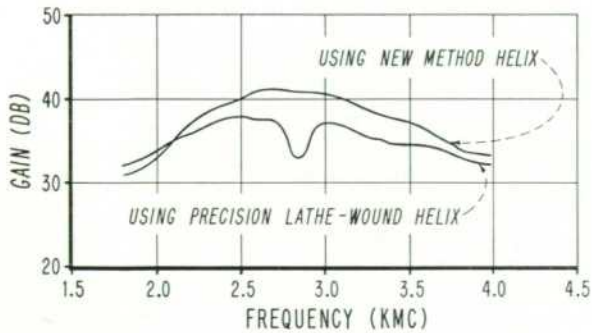
Fig. 1. Helices formed by new methods typically give higher gains and smoother characteristics than precision lathe-wound helices as shown in above curves.
