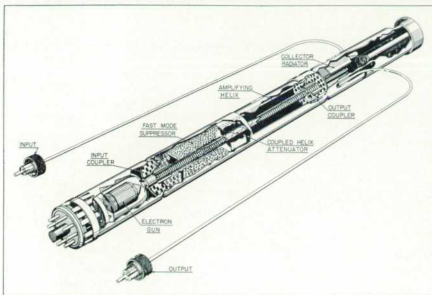
Fig. 8. Encapsulated tube assembly.
