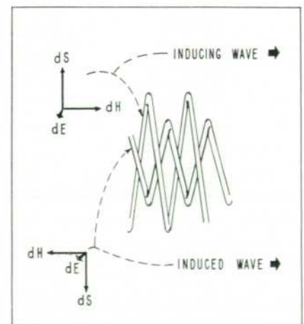
Fig. 7. Sketch showing how opposite senses of winding of coupling and tube helices cause induced wave to travel in same direction as inducing wave.
