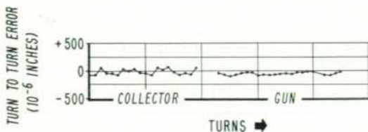
Fig. 2. Error measured on typical helix formed by new method. Samples near gun and collector ends of helix are shown.
