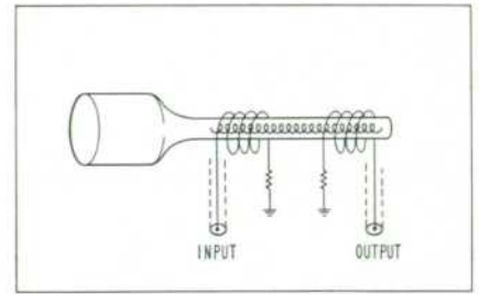
Fig. 6. Schematic arrangement of input and output couplers. A third coupler wound from resistance wire is used for attenuation of backward wave.
