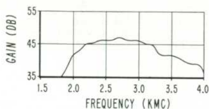
(a) Small signal gain (-35 dbm input)
