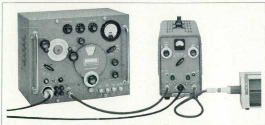
Fig. 1. New hp- Model 491A 2-4 kmc Traveling-Wave Tube Amplifier (center) used with -hp- 616A UHF Signal Generator to form 1 watt signal source. Ten milliwatt TWT amplifier is similar in appearance to 1 watt unit shown.
