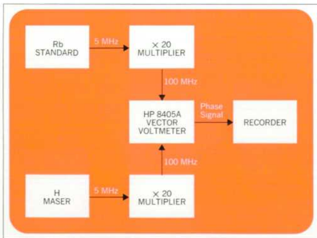
Fig. 9. Equipment arrangement used in making record of Fig. 8.
