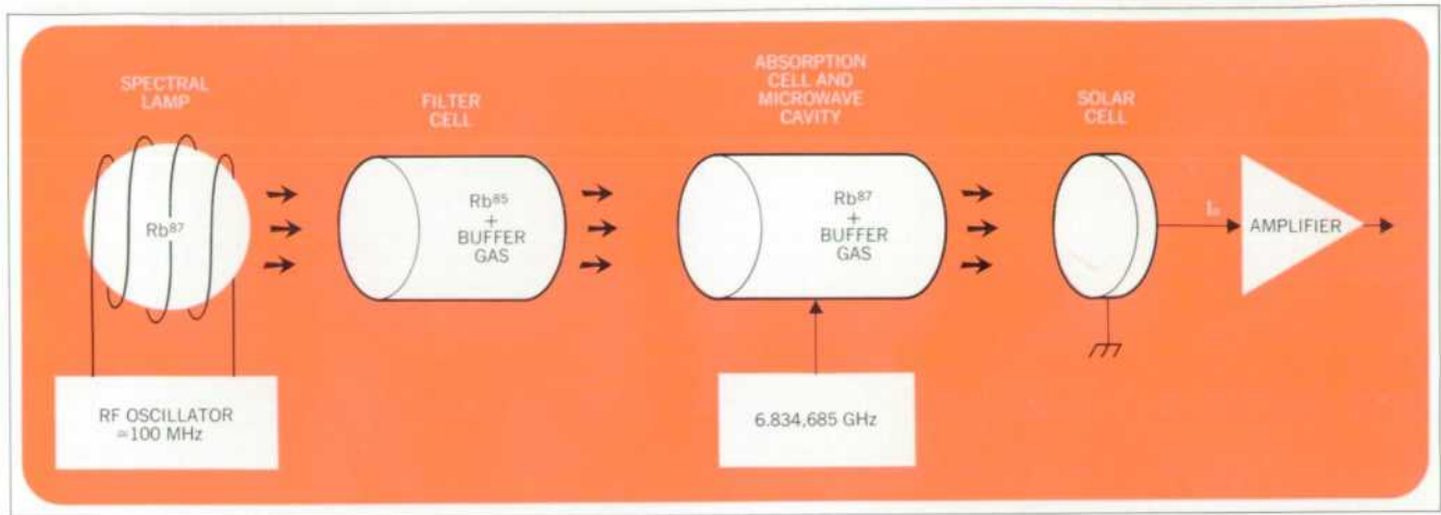
Fig. 6. Schematic representation of rubidium-vapor cell arrangement.
