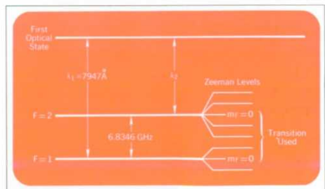
Fig. 7. Simplified diagram of the energy levels of \text{Rb}^{87} which are of significance in operation of cell.
