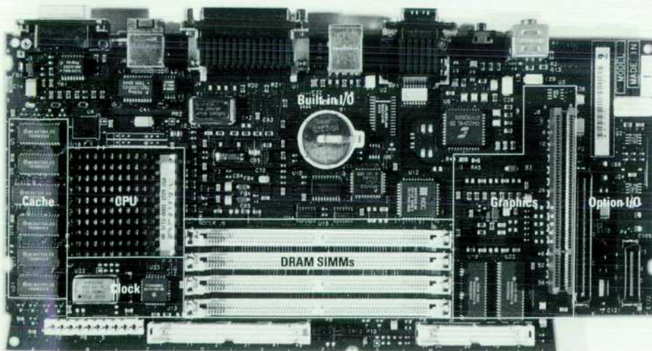
Fig. 3. The Model 712 system board.
