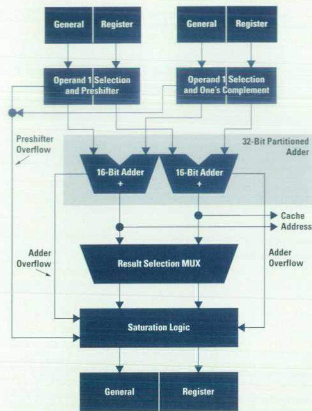
Fig. 3. Flow of halfword instructions showing the location of the saturation logic in relation to the ALU.
