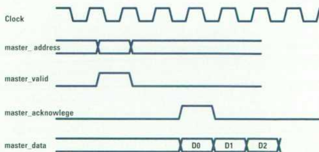
Fig. 3. Master read timing diagram.
