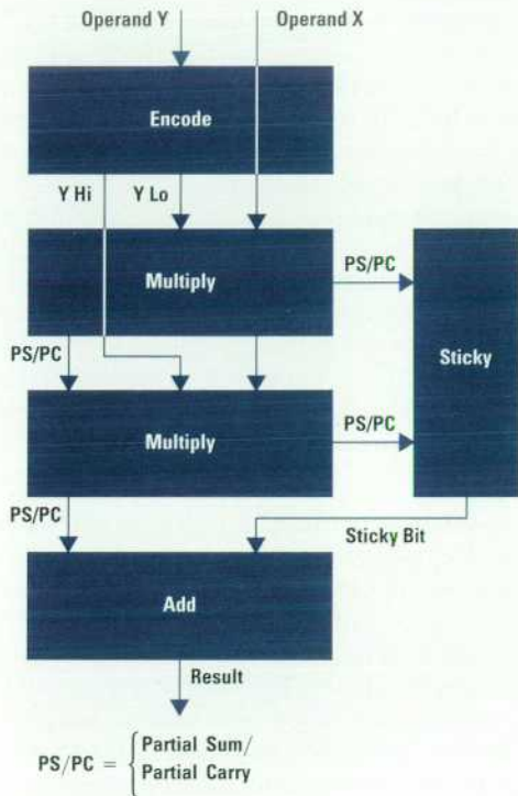
Sticky computes the sticky bit, which is part of the IEEE floating-point standard. The two multiply blocks perform the bulk of the computation. (a)
