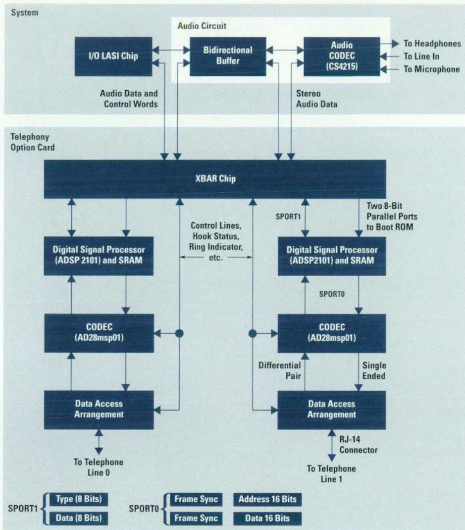
Fig. 1. Block diagram of HP TeleShare.
