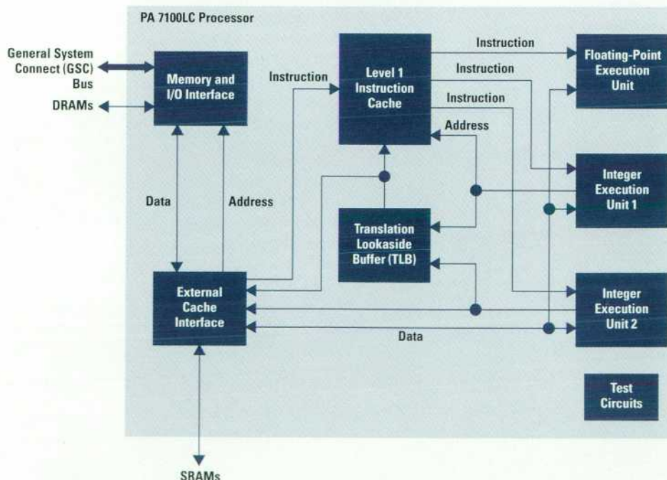
Fig. 1. A simplified block diagram of the PA 7100LC processor.
