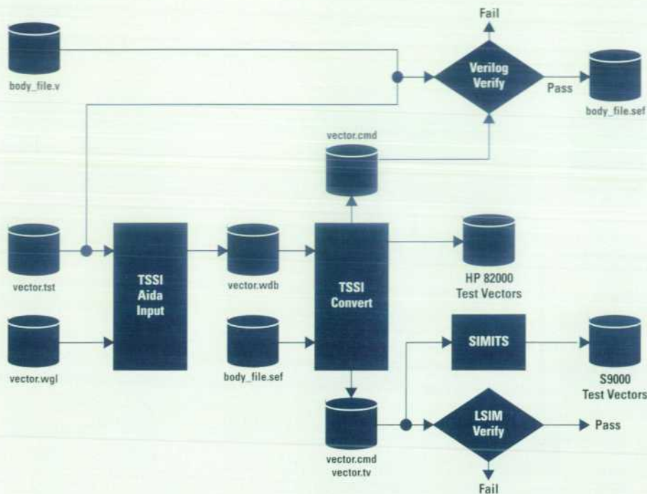
Fig. 4. Vector verification and tester translation tools flow. TSSI is a test program generation tool from TSSI, Inc. Aida represents a suite of test tools from Aida, Inc. LSIM is a special FET-level simulator. SIMITS is a format conversion tool from Schlumberger.
