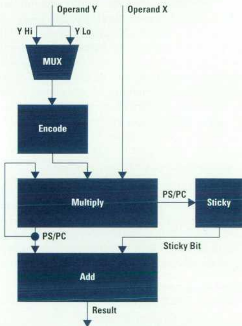
Sticky and PS/PC are the same as above. Partial results iterate through the single multiply block. (b)
