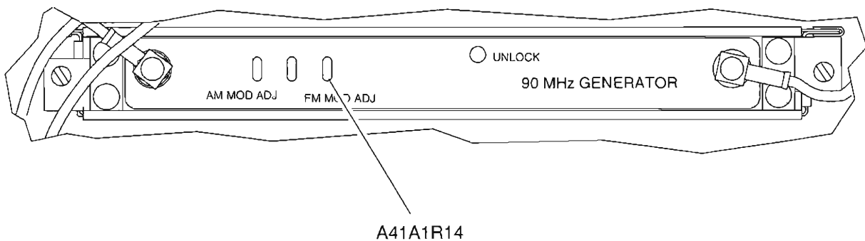
Figure 1-26 90 MHz Generator PC Board Assembly (34A5A41A1) Calibration Points
