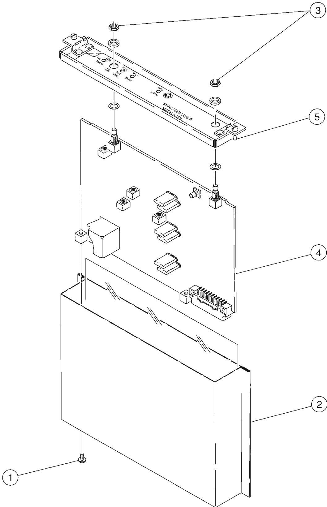
Figure 1-37 Analyzer Log/IF PC Board Assembly (34A5A7A1) Removal
