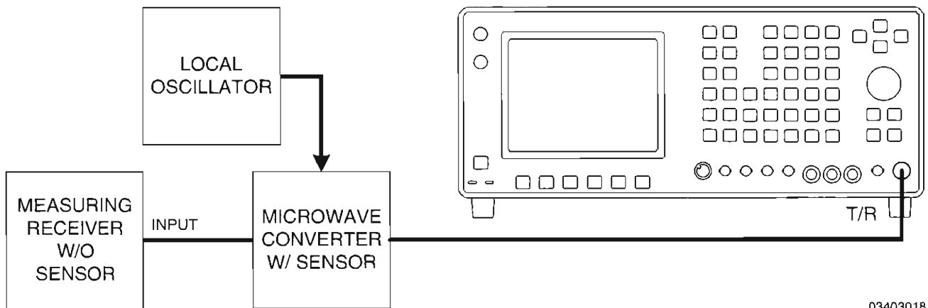
Figure 1-25 Generator FM Deviation Calibration Hook-Up
