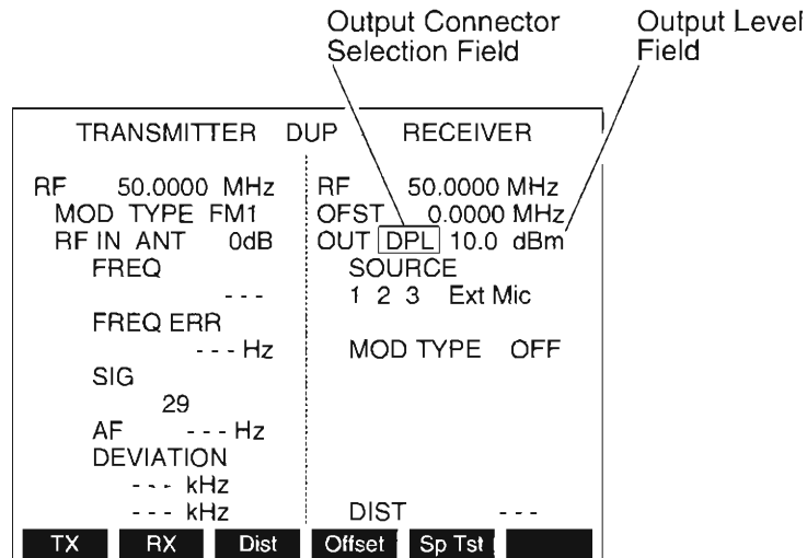
Figure 1-21 Duplex Operation Output Connector Selection Field
