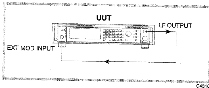
Fig. 7-19 SINAD test set-up
