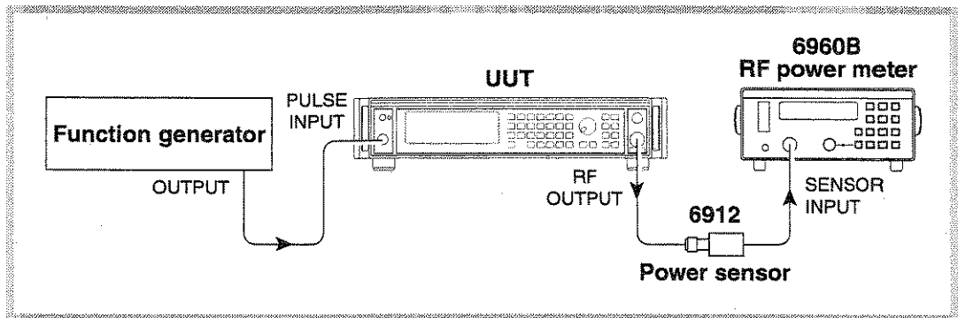
Fig. B-7 Pulse modulation test set-up
