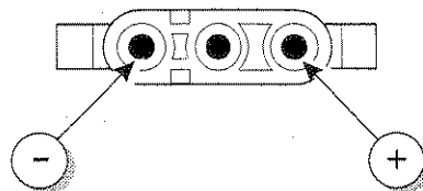
Fig. 2-1 DC input socket showing connector polarity (viewed from rear of instrument)
