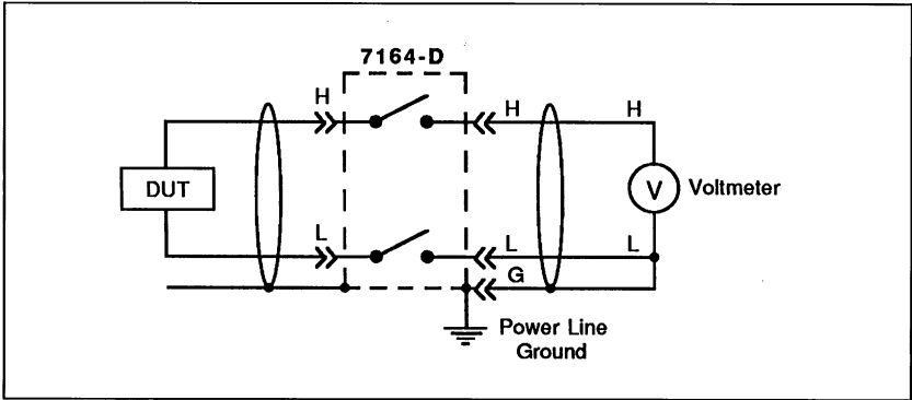
Figure 2-3. Shielded Measurement
