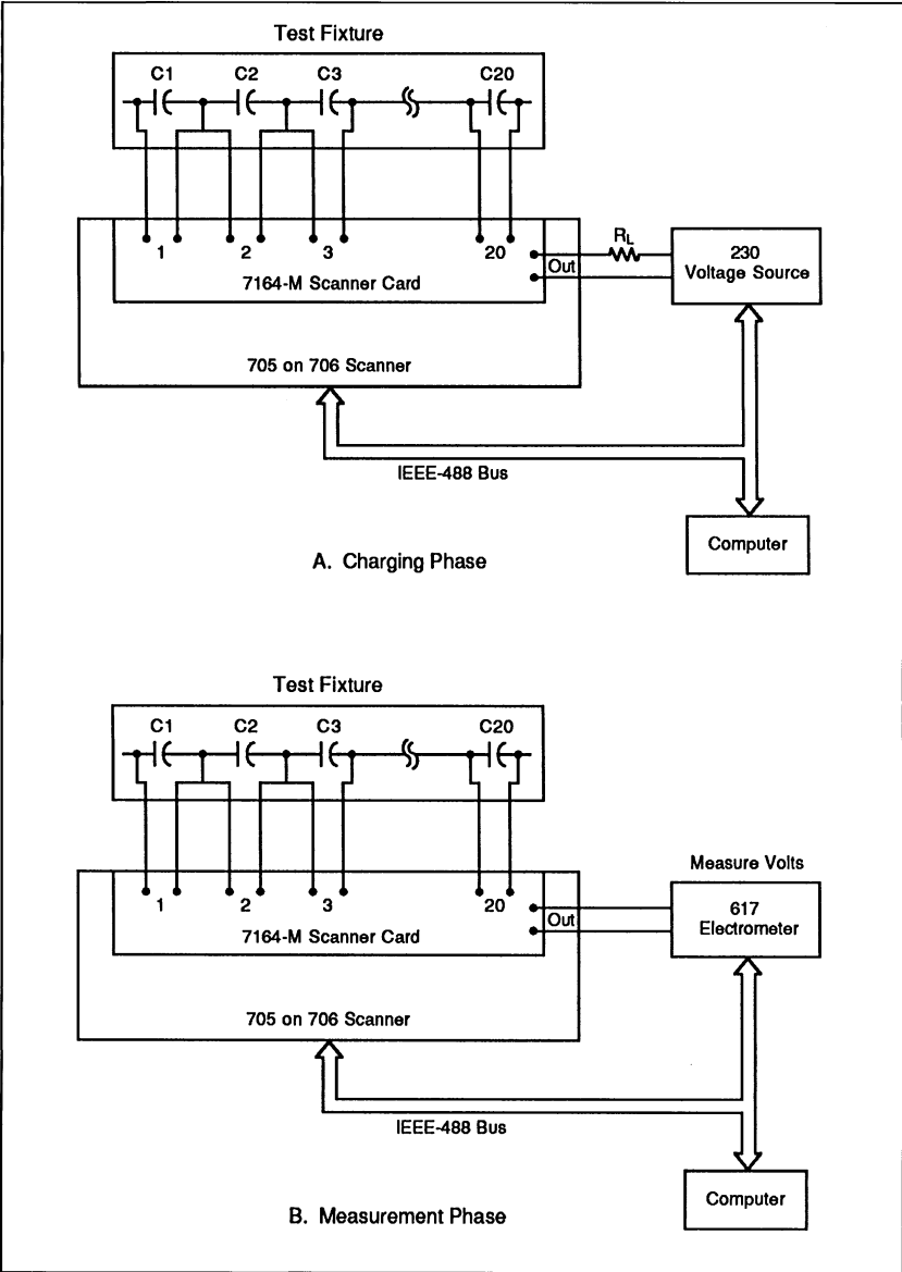
Figure 3-3. Capacitor Testing
