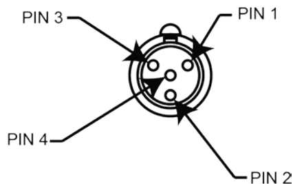
Figure 1: Model 8020 interlock expansion termination plug pinouts
