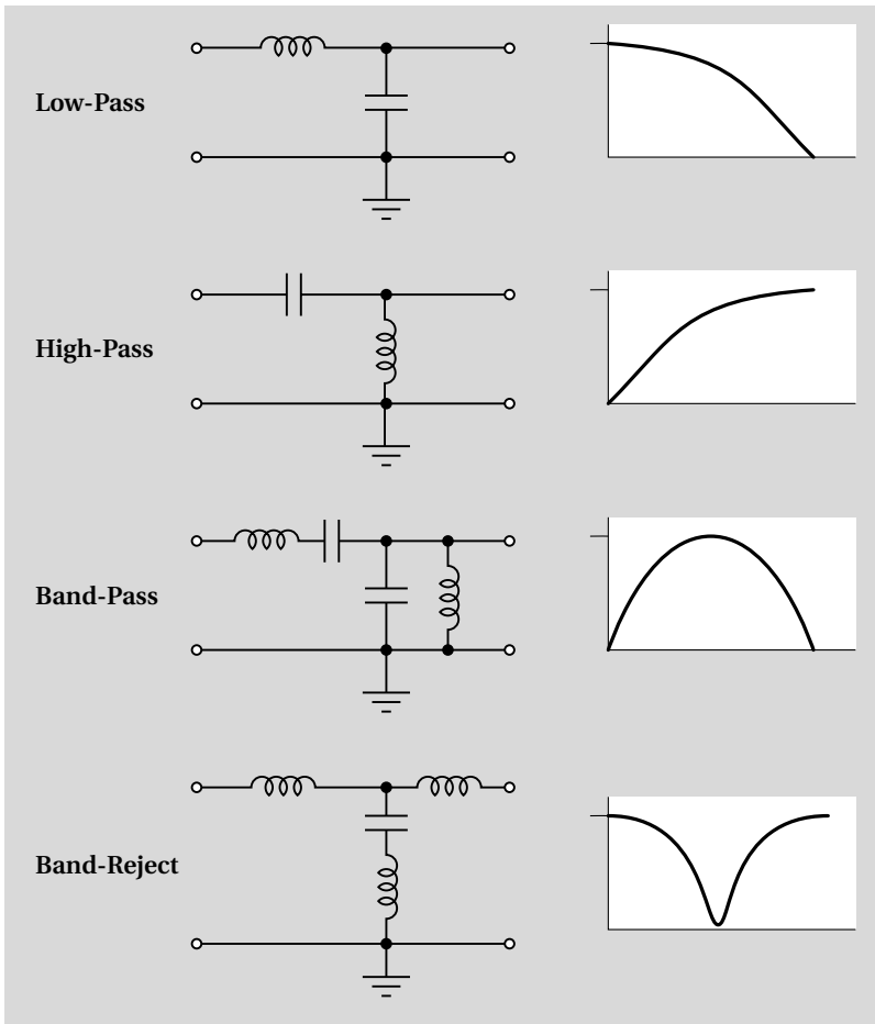
Figure 4-17. Passive L-C filter designs
