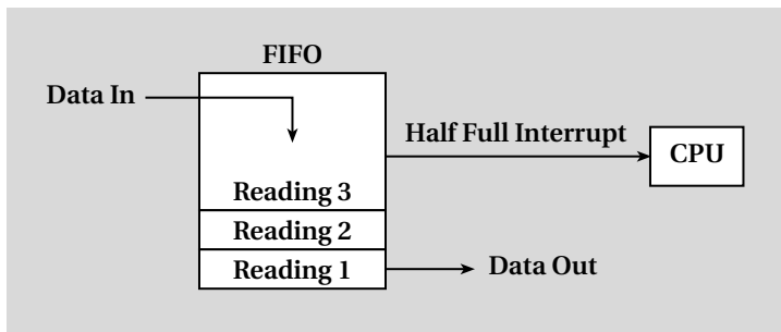
Figure 3-3. FIFO operation
