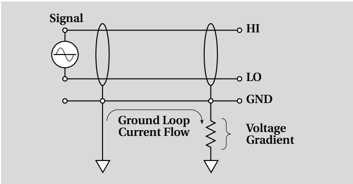
Figure 4-13. Ground loop
