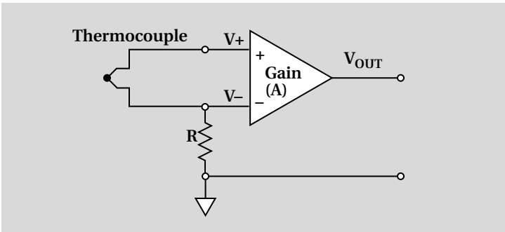
Figure 4-14. Thermocouple A/D input with ground return resistor (R)
