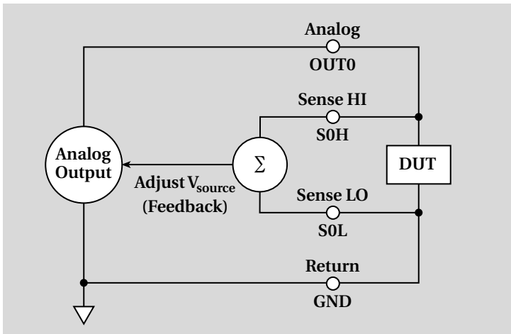
Figure 9-7. Analog output with four-wire remote sense
