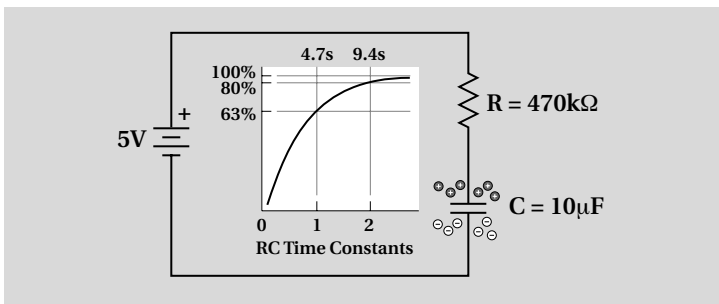
Figure 4-7. RC time constant
