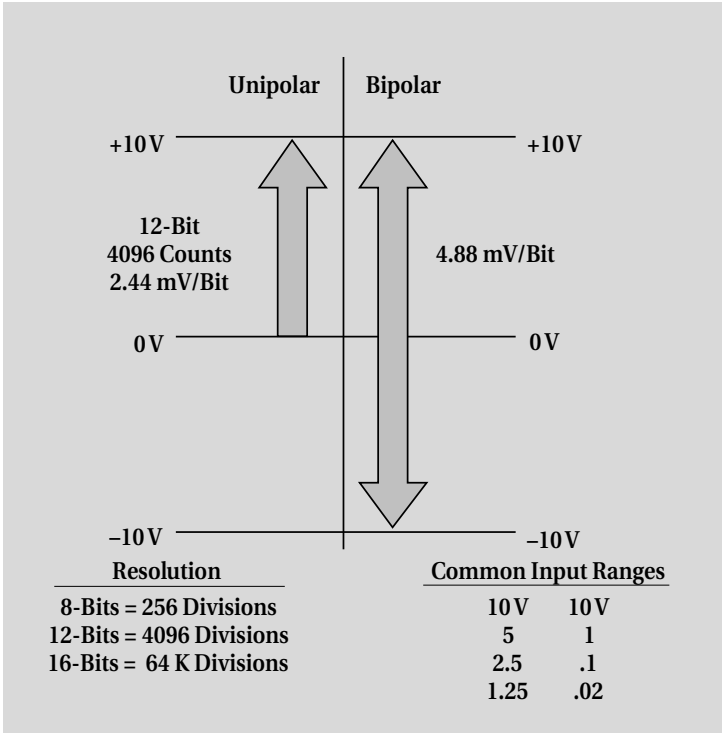
Figure 4-15. Bipolar and unipolar input ranges
