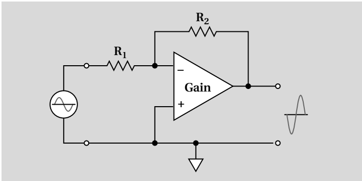
Figure 4-10. Inverting amplifier
