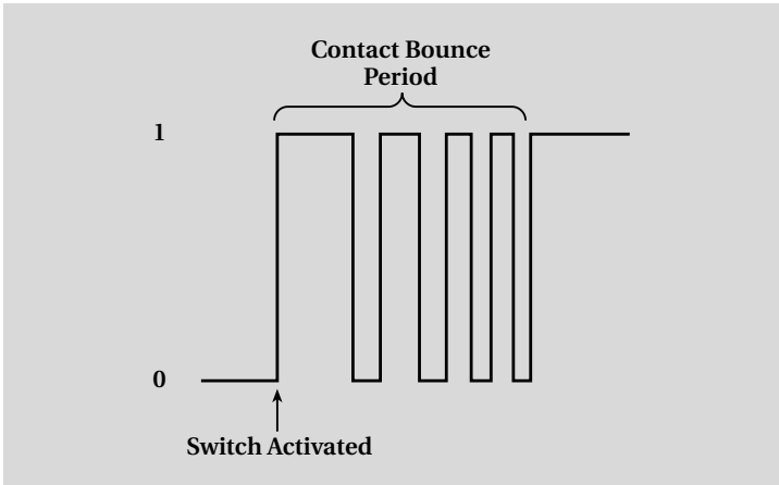
Figure 5-4. Contact bounce
