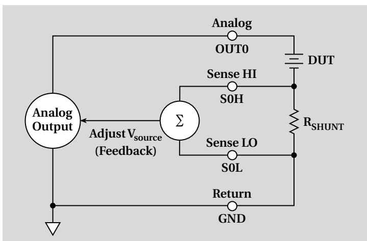
Figure 9-10. Constant current battery test configuration
