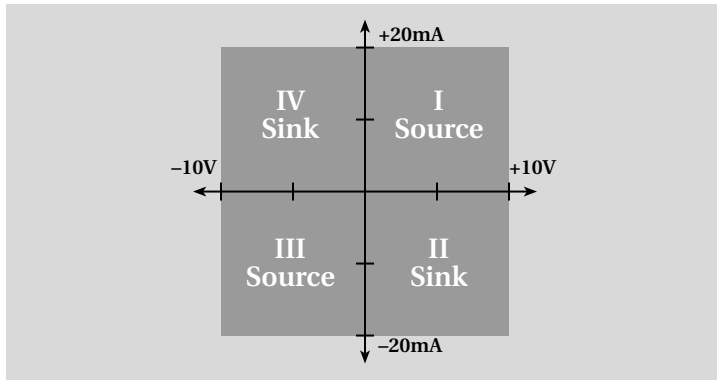
Figure 9-8. Four-quadrant operation
