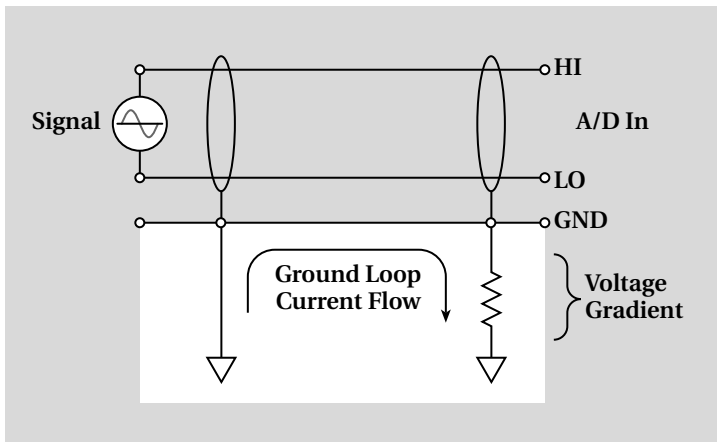
Figure 5-11. Ground loop
