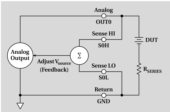
Figure 9-11. Constant voltage battery test configuration
