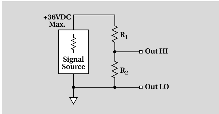
Figure 4-2. Voltage divider
