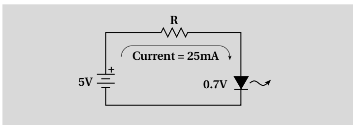
Figure 4-1. Current limiting
