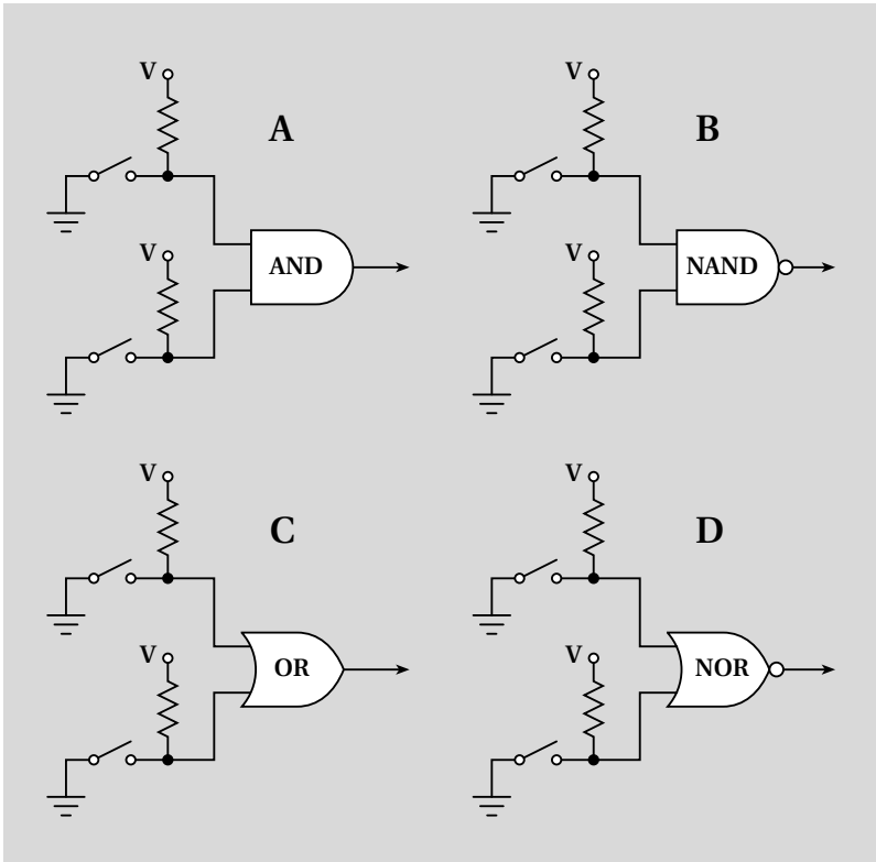
Figure 4-18. Digital gates
