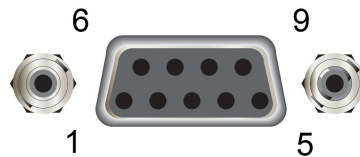
Figure 111: Model 2460 digital I/O port
