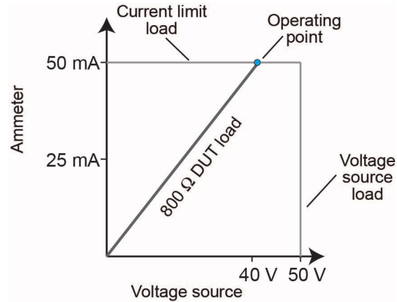
Figure 131: Model 2460 current limit boundary example limited
