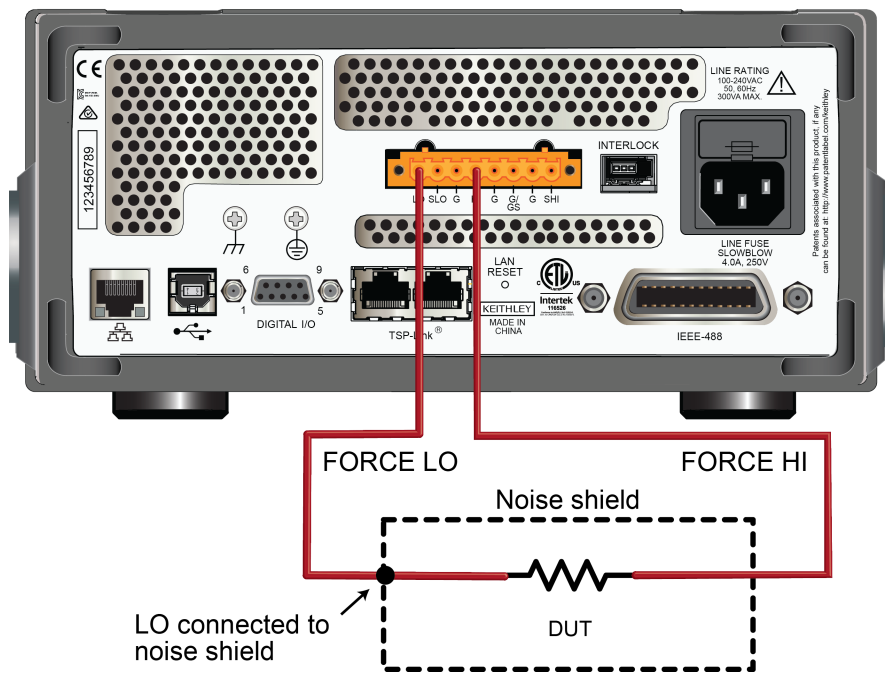
Figure 132: Model 2460 rear-panel noise shield connections
