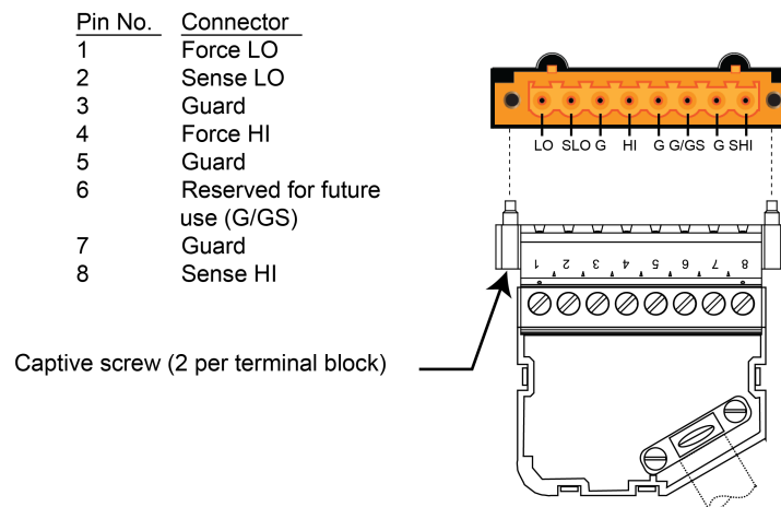
Figure 56: Model 2460 rear-panel screw terminal connections
