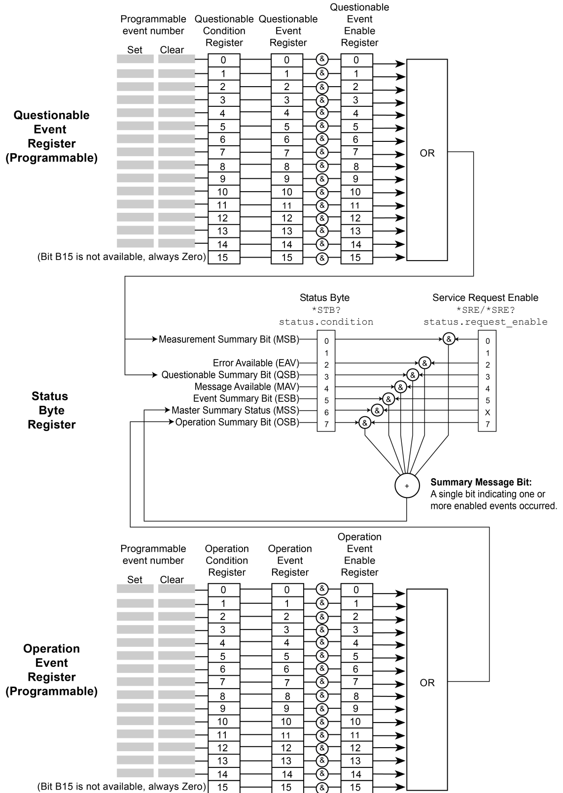
Figure 167: Programmable status registers diagram
