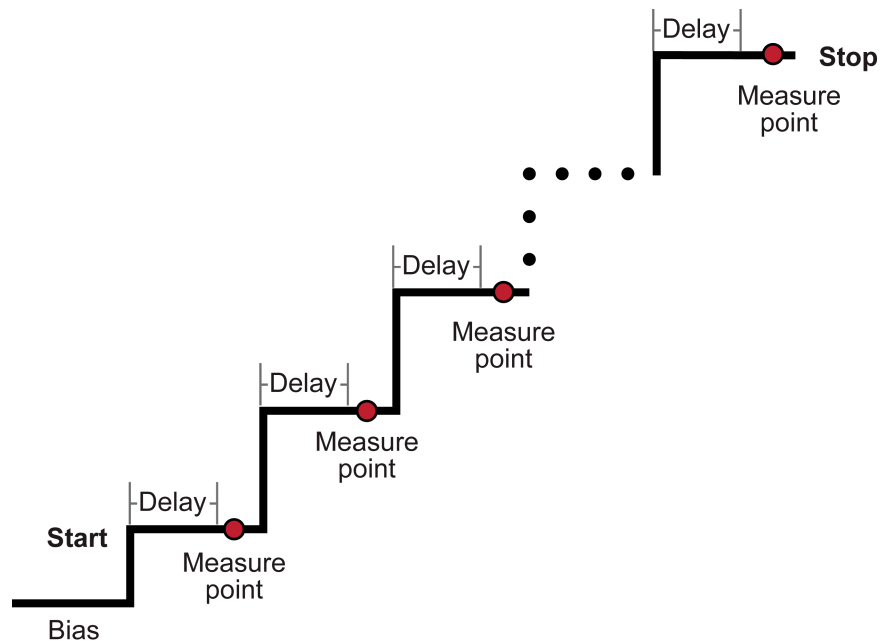
Figure 107: Model 2460 sweep linear staircase
