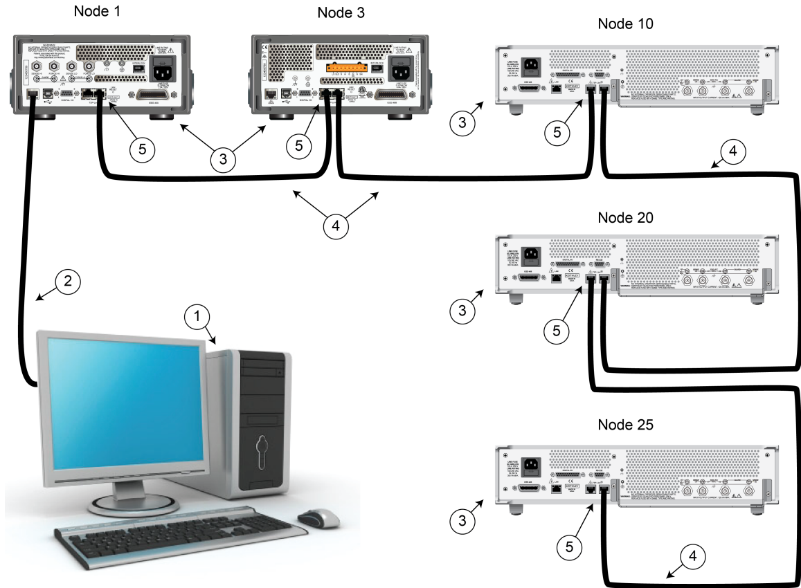
Figure 123: TSP-Link connections
