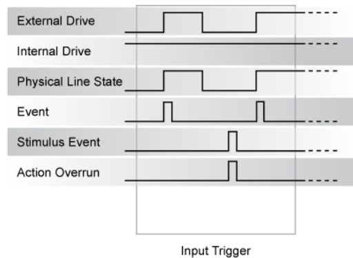
Figure 114: Synchronous master input trigger
