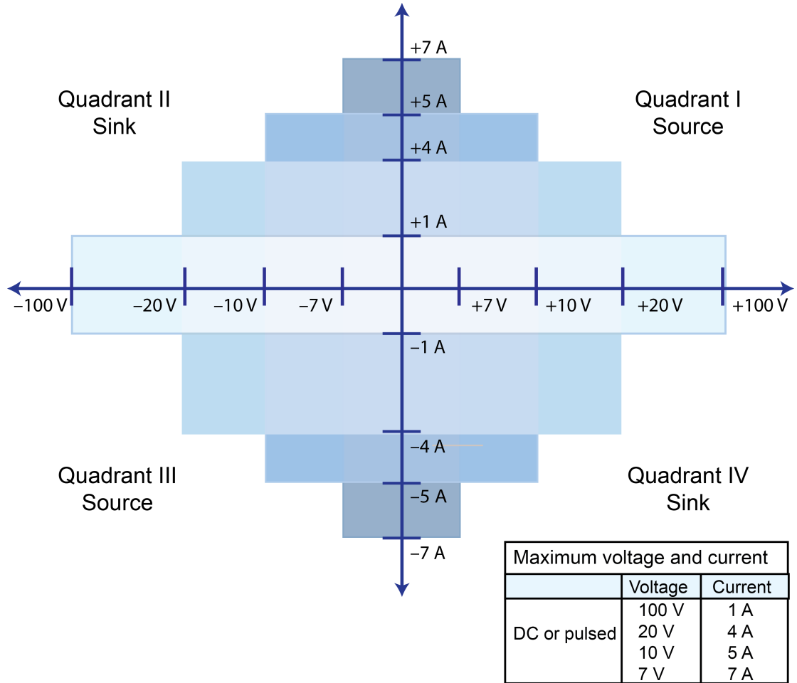
Figure 126: Model 2460 operating boundaries
