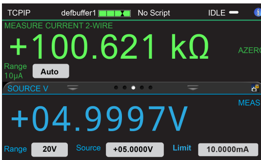
Figure 66: Resistance measurement using SVMl and reading ohms
