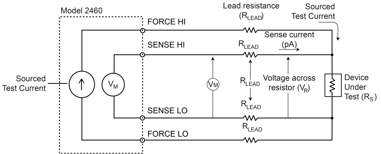
Figure 64: Model 2460 4-wire resistance sensing.png
