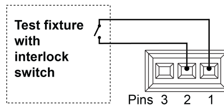
Figure 58: Model 2460 interlock pins
