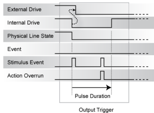
Figure 115: Synchronous master output trigger
