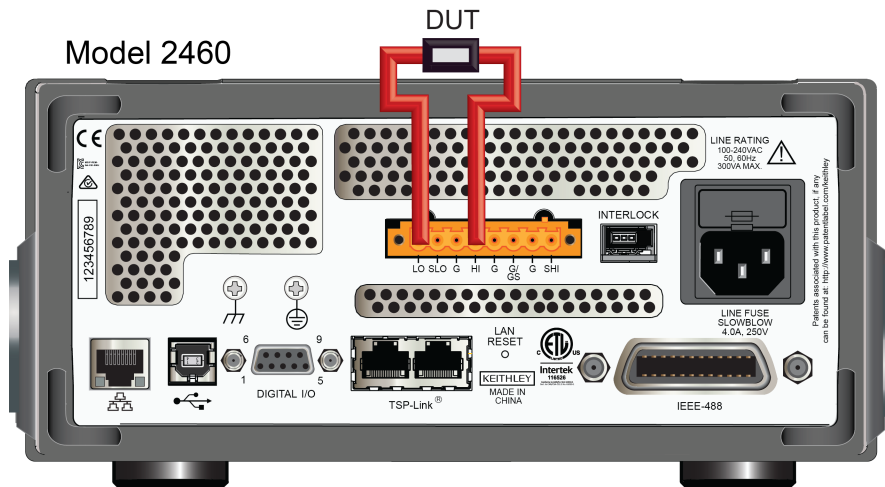
Figure 60: Model 2460 2-wire rear panel connections
