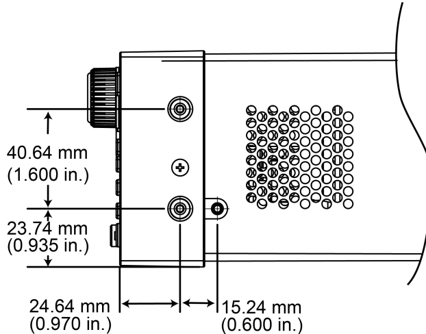
Figure 34: Model 2460 mounting screw locations and dimensions
