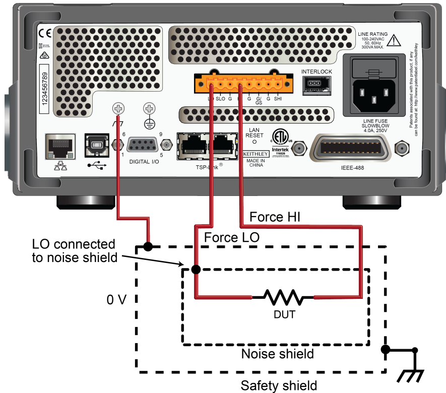
Figure 133: Model 2460 rear panel noise shield
