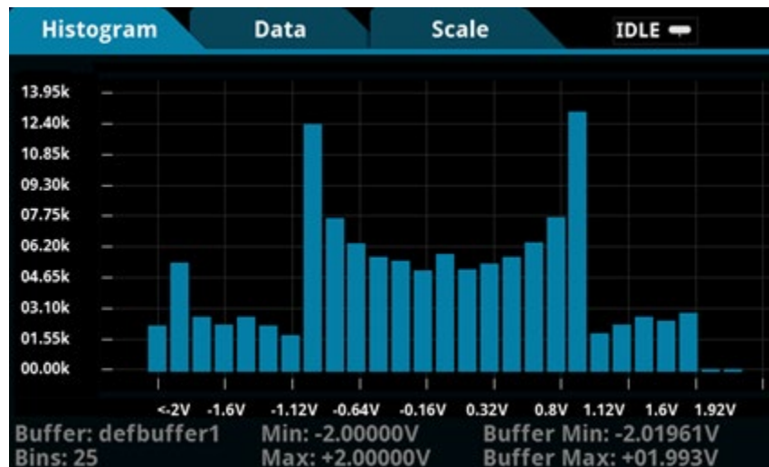
Figure 24: Model 2460 Histogram
