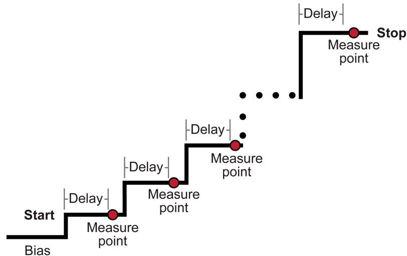
Figure 108: Logarithmic staircase sweep
