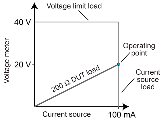
Figure 128: Model 2460 limit boundary example — normal
