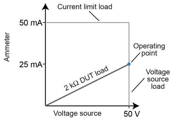
Figure 130: Model 2460 current limit boundary example normal
