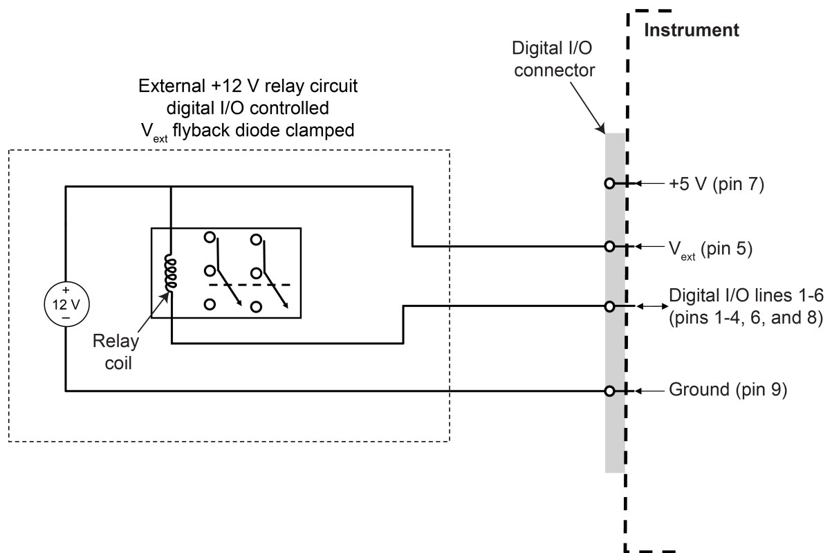
Figure 113: Digital I/O Vext (example external circuit)
