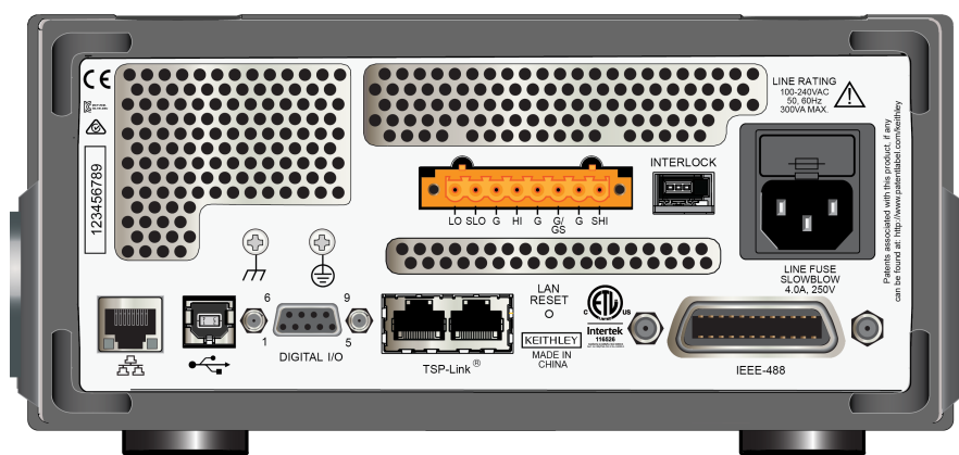
Figure 1: Model 2460 rear panel
