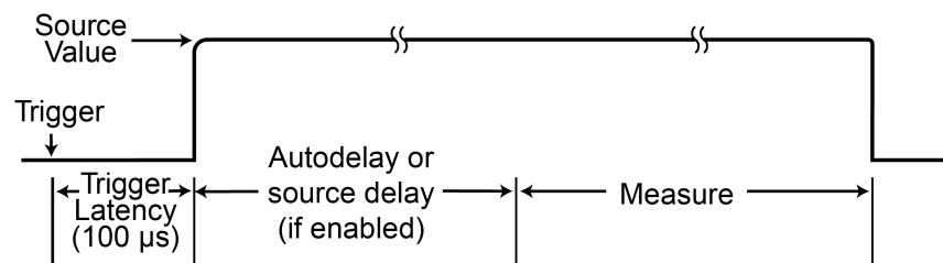
Figure 72: Model 2460 settling and delay times
