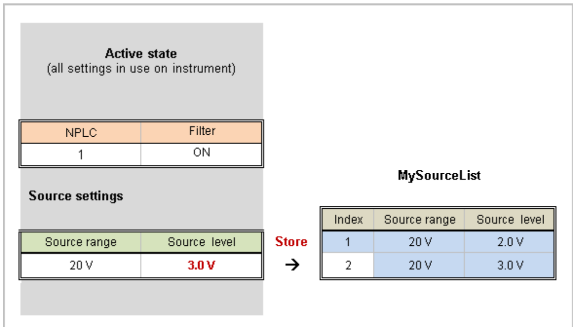
Figure 103: Example configuration point 2
