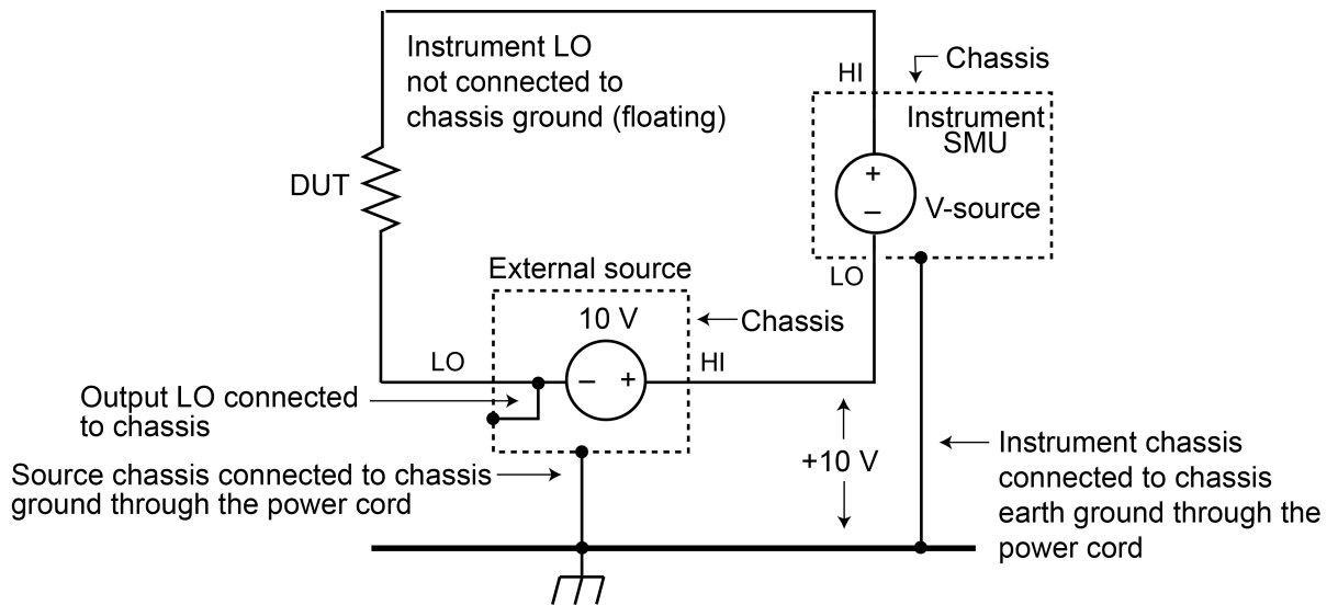
Figure 134: Floating the instrument schematic
