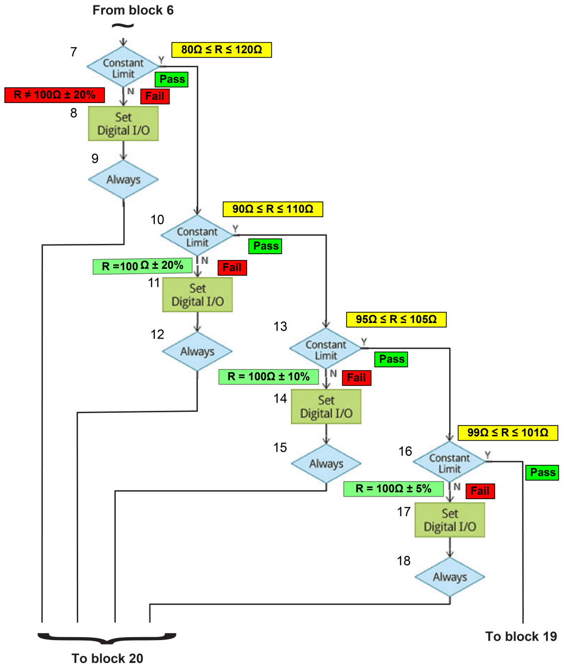
Figure 120: Resistor grading example blocks 7 to 18
