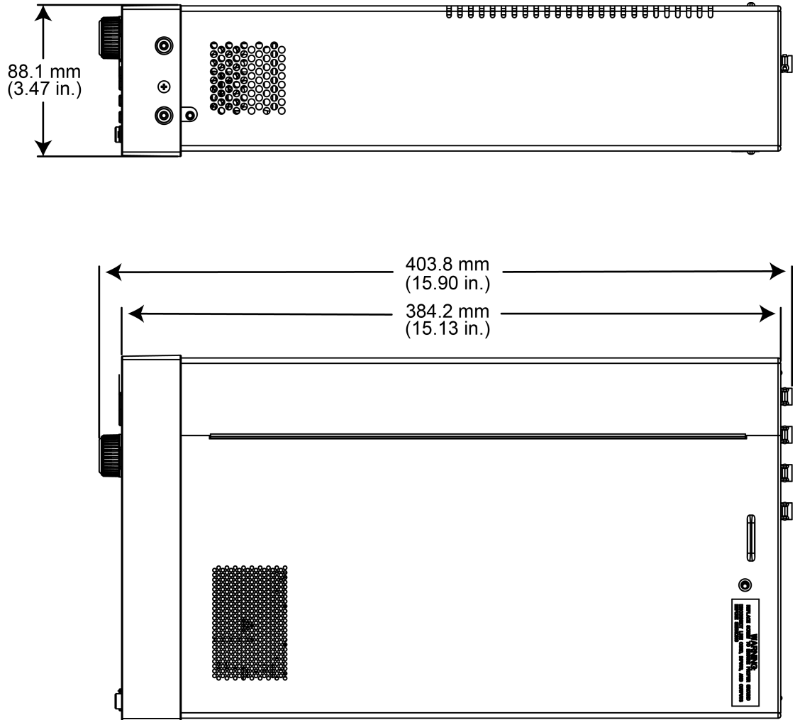
Figure 38: Model 2460 top and side dimensions with handle and bumpers removed
