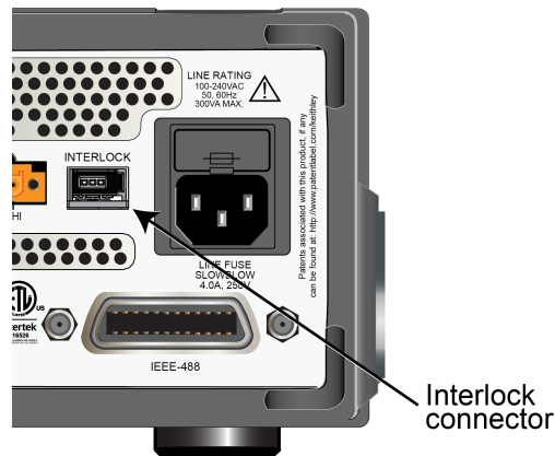
Figure 57: Model 2460 rear-panel interlock location
