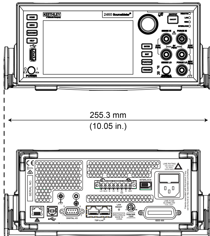
Figure 35: Model 2460 dimensions front and rear with handle and bumpers
