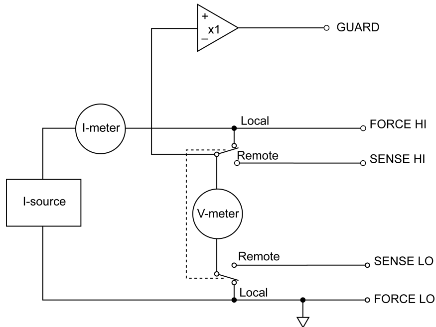
Figure 124: Current source configuration
