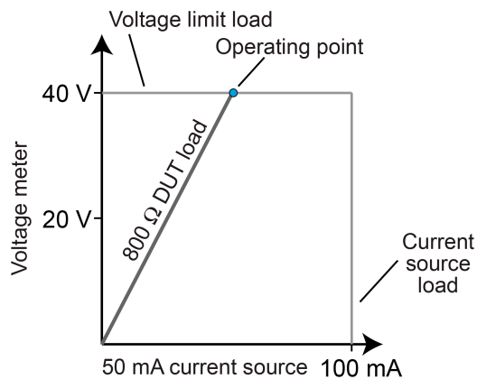
Figure 129: Model 2460 limit boundary example when limited
