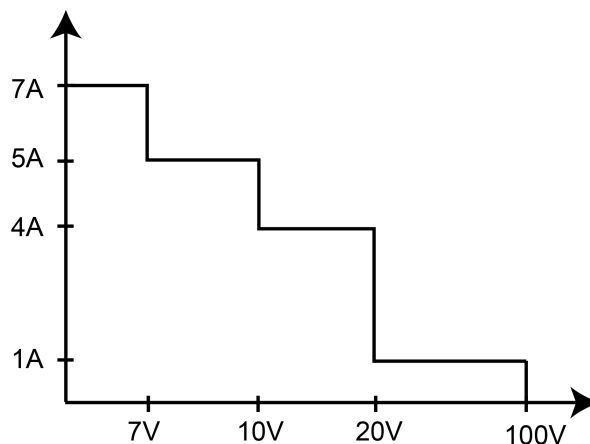
Figure 127: Model 2460 current source output characteristics
