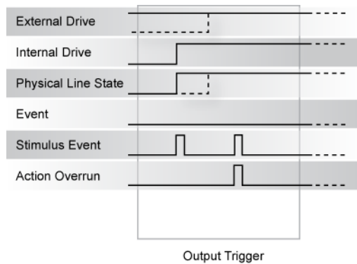
Figure 117: Synchronous acceptor output trigger
