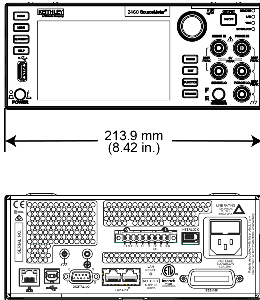
Figure 37: Model 2460 front and rear panel dimensions with handle and bumpers removed
