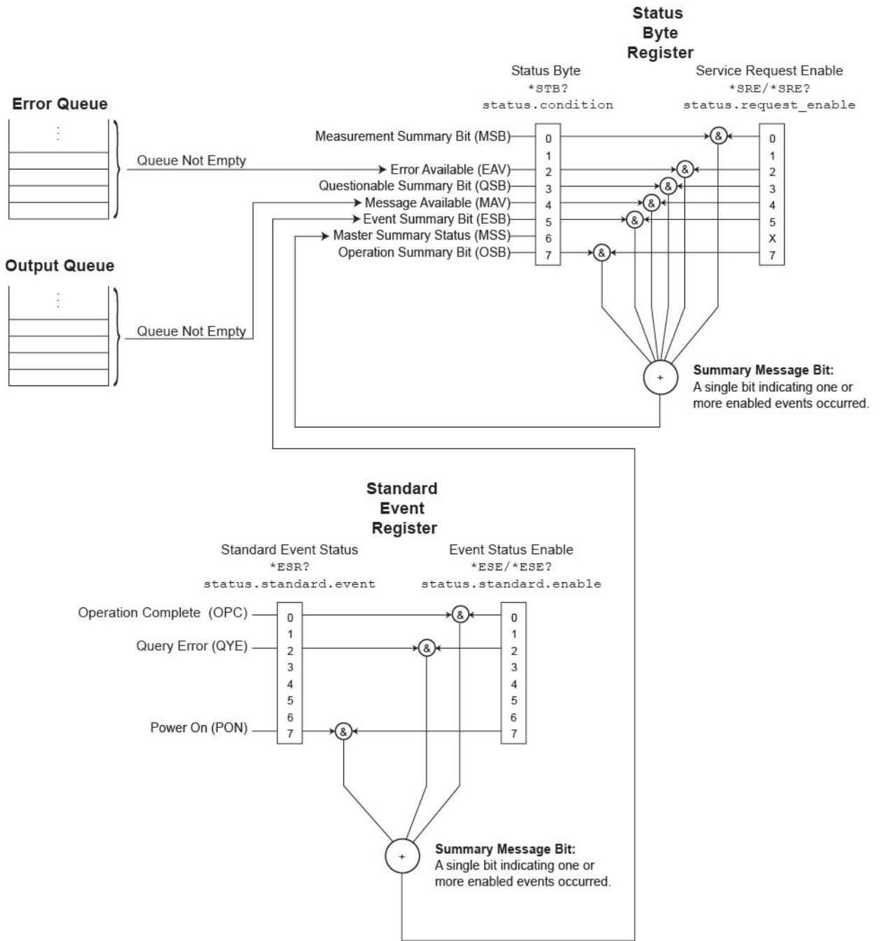
Figure 165: Non-programmable status registers diagram
