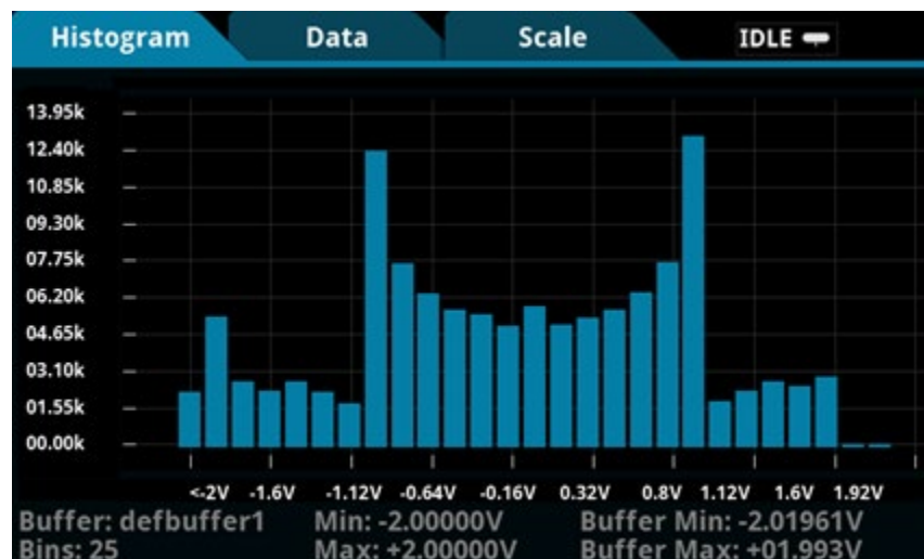
Figure 77: Model 2460 Histogram
