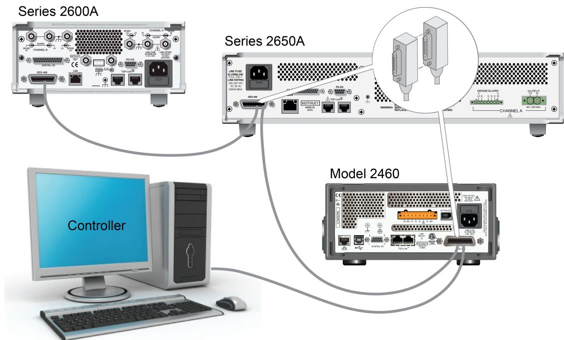
Figure 40: Model 2460 IEEE-488 connections
