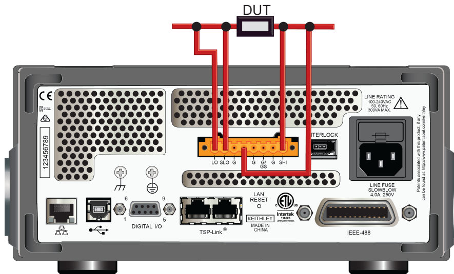
Figure 61: Model 2460 rear panel 4-wire remote sense connections
