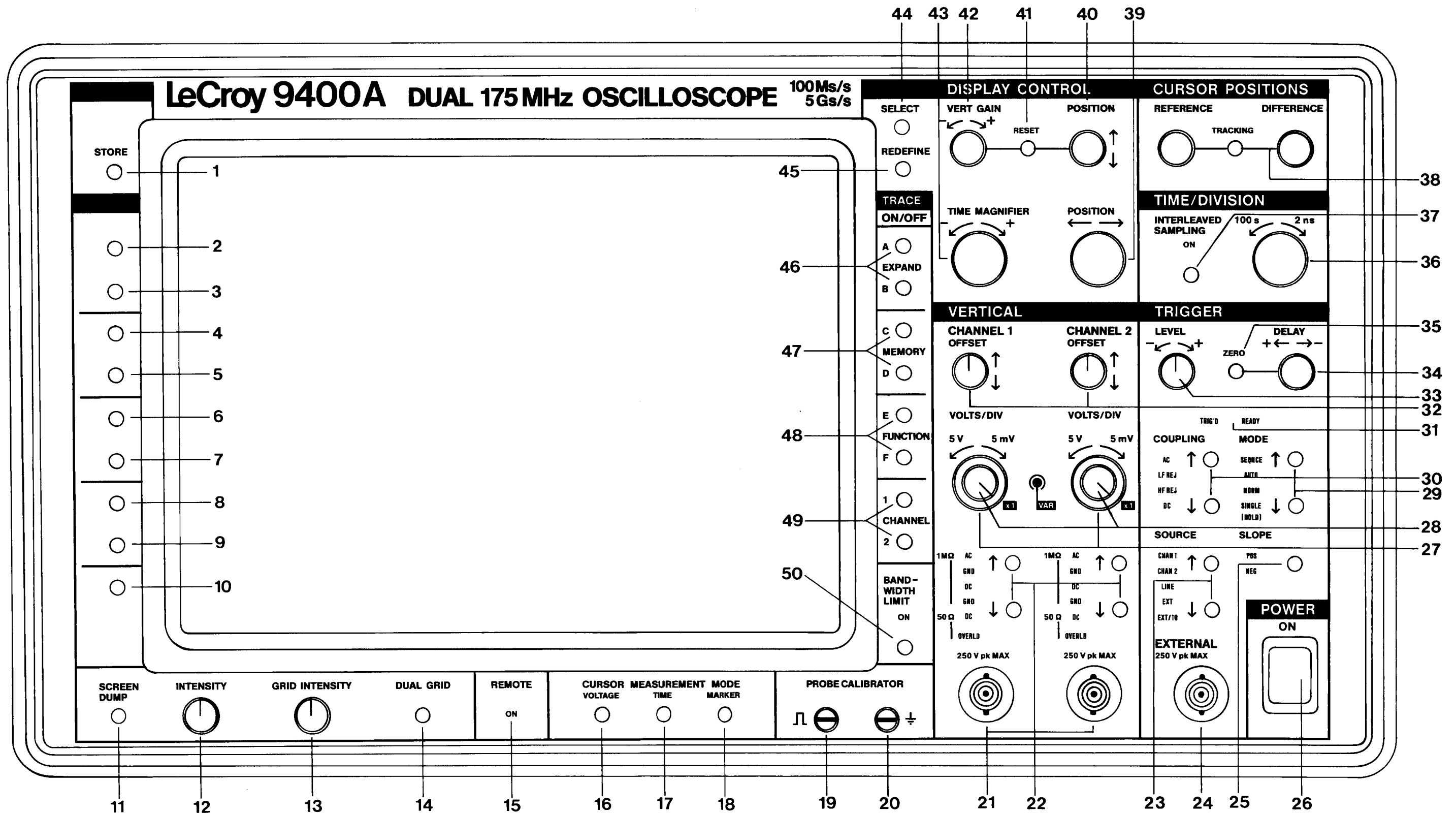
9400A FRONT PANEL Figure 1.1
