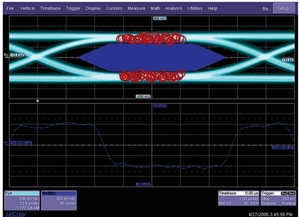
Observe bit sequences that cause mask violations.
