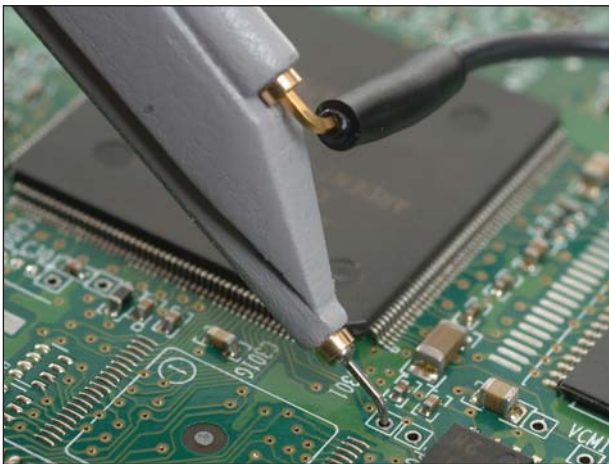
Hard-to-reach spaces can be probed with the Bent Sharp Tip and can be used with a range of ground leads like the flexible Short Right-angle Lead shown here.
