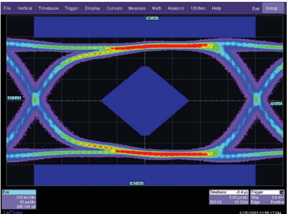
Eye pattern of serial ATA signal.
