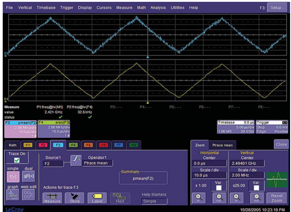
See multiple cycles of spread spectrum clocking.
