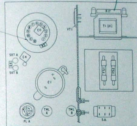
VIEW IN DIRECTION OF ARROW 'B'
