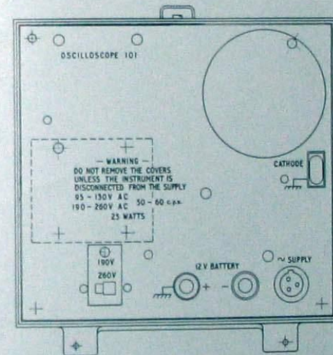
VIEW ON REAR PANEL
