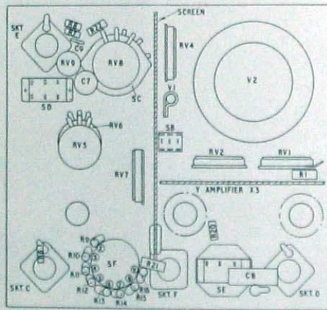
VIEW IN DIRECTION OF ARROW 'A'
