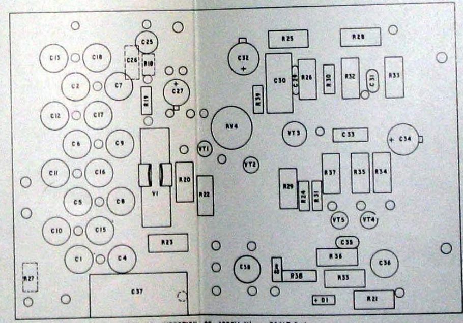
Y AMPLIFIER COMPONENT LAYOUT
