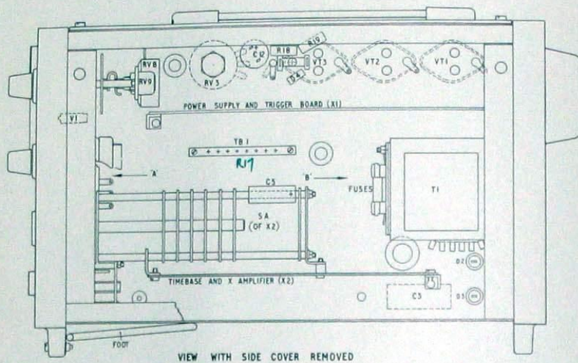
VIEW WITH SIDE COVER REMOVED
