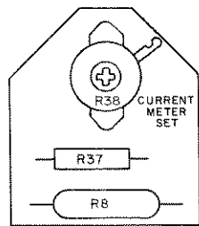
LOCATION OF COMPONENTS METER BOARD
