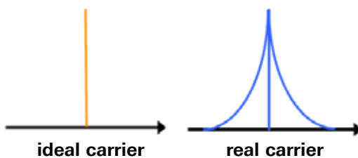
An ideal carrier would have no phase noise, but a real signal would look like this.
