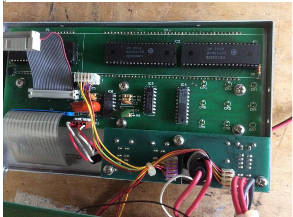
Sencore LC102 Display Board.JPG (197.63 kB, 720x538 - viewed 392 times.)
