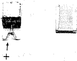
Fig. 45 — A tantalum chip capacitor (left) can be identified from a ceramic chip capacitor by its positive lead.
