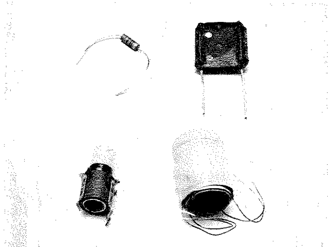
Fig. 51 — Air and ferrite core inductors are tested with the "coil" component type switch selected.
