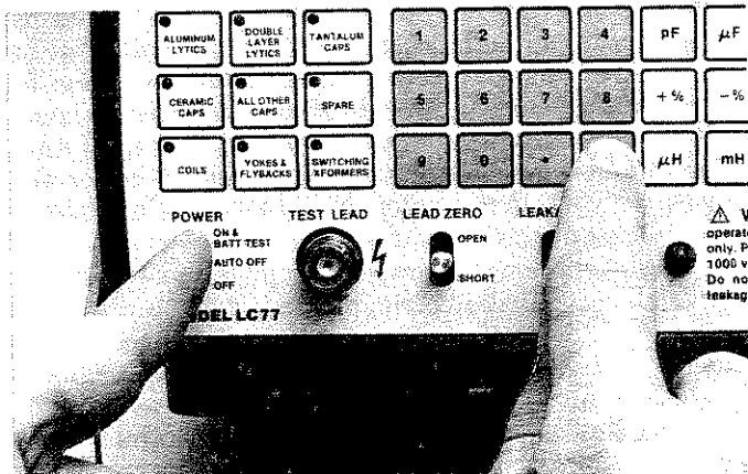
Fig. 67 — Push the "CLR" button while holding the power switch to "ON & BATT TEST" to check LCD display.
