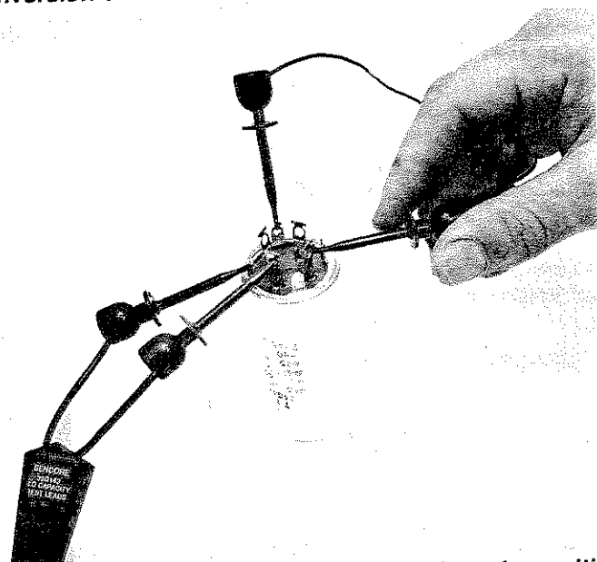
Fig. 54 — Test the leakage of one section of a multi-section lytic, then short one of the remaining sections to ground. Any increase in leakage current indicates leakage between that section and ground.
