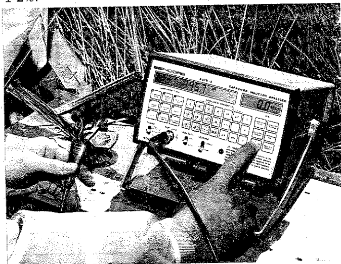
Fig. 64 — Use the LC77 to measure the distance to breaks or shorts in buried cable.
