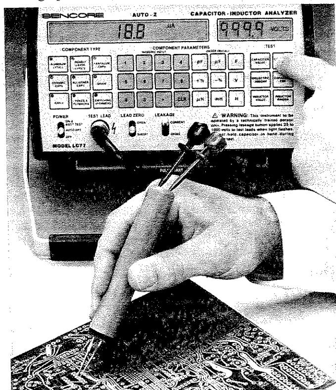
Fig. 65 — Small leakage paths can be detected with the LC77 Hi Pot test.
