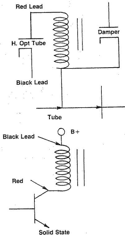
Fig. 60 — Connect to the primary side of a flyback to do the ringing test.
