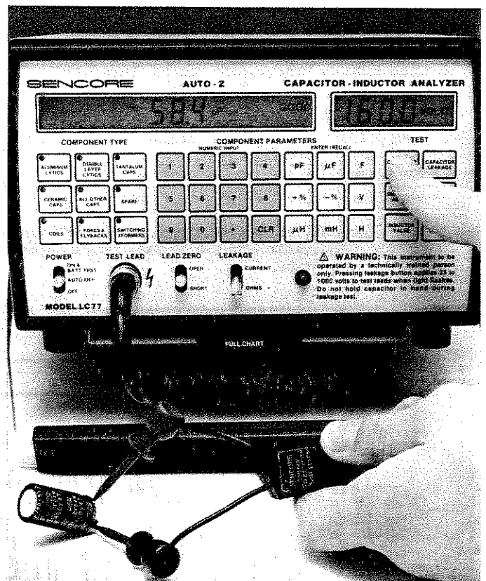
Fig. 20 — The LC77 provides an automatic good/bad indication of each capacitor parameter.
