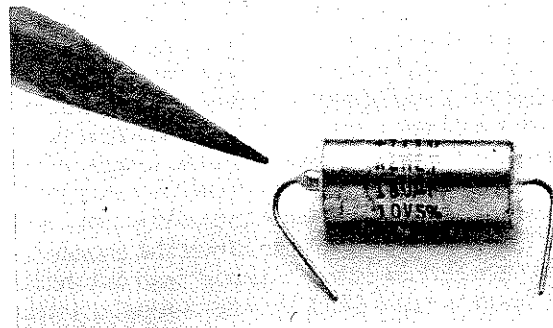
Fig. 43 — Axial lead tantalum capacitors, like the one shown here, are easily identified from axial lead aluminum electrolytics by a solder weld on one end.
