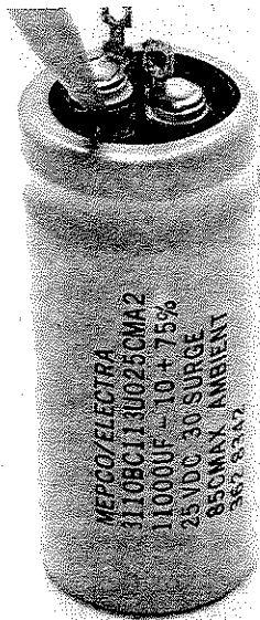
Fig. 42 — All aluminum electrolytics have a rubber seal.
