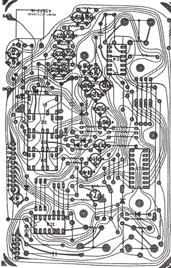
Foil Side
