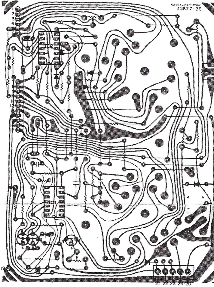
Foil Side
