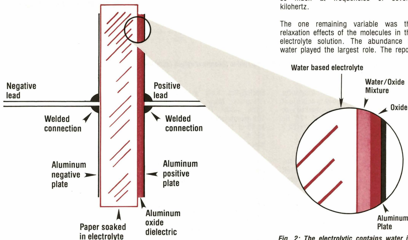
Fig. 2: The electrolytic contains water in the paper spacer and part of the oxide layer. This water causes the value to change with frequency.
