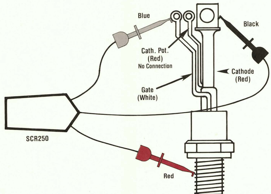
Fig. 6: Connect the SCR250 test leads up to large stud mount SCRs following the color coding shown here.
