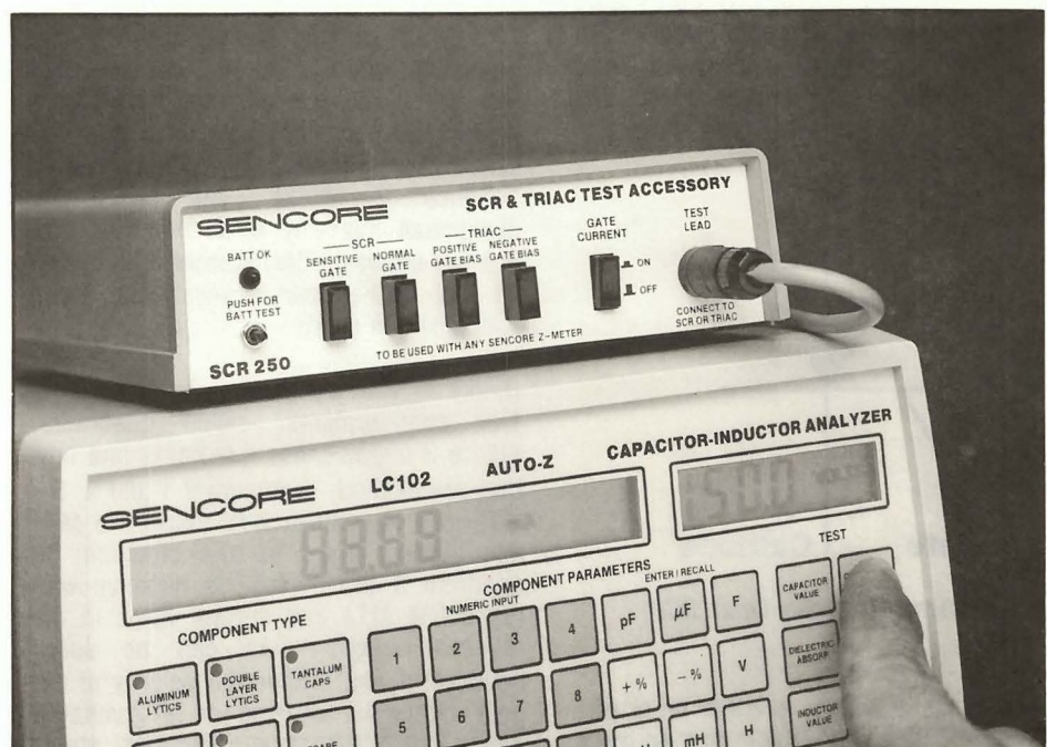
Fig. 4: The SCR250 can be mounted on top of a Z Meter using Velcro strips supplied with the SCR250.
