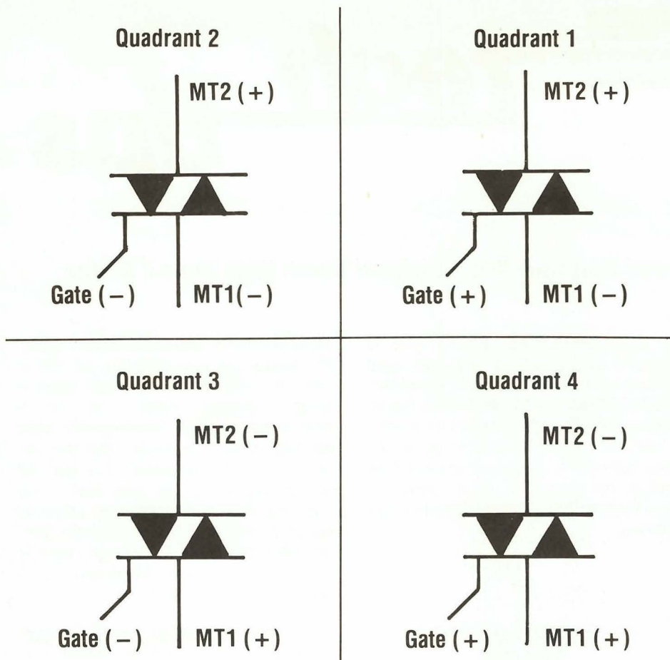
Fig. 3: A triac can operate under four different voltage polarity conditions. Quadrant I and III are the most common.
