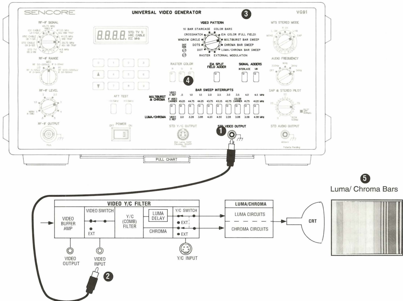
Fig. 3: The Luma/Chroma Bar Sweep pattern dynamically tests the separation and overall frequency response of the Comb filters.
