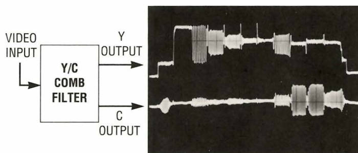
Fig. 4: Set the comb filter to null the chroma observed in the luminance bars and luminance interference to the chroma bars while obtaining best overall chroma and luminance frequency response as shown here.
