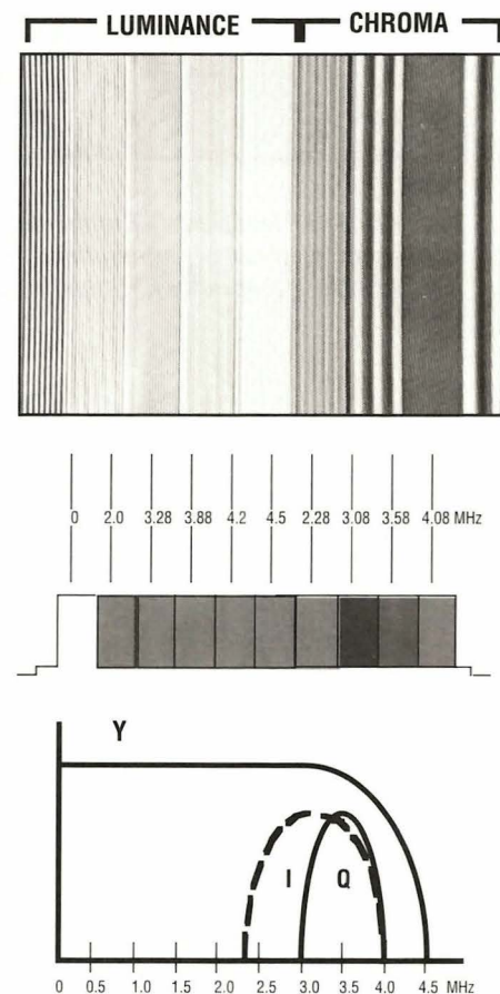
Fig. 1: The Luma/Chroma Bar Sweep video pattern includes luminance and chrominance frequency bars to dynamically test the separation and frequency response of comb filters.
